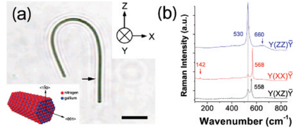
Figure 1. (a) Video image and polarization configuration of the Raman instrument. The Y direction is labeled for the incoming laser where Z and X define polarizations parallel and perpendicular to the wire growth direction, respectively. Scale bar = 5 \mu\text{m} . Inset: Illustration of crystallographic directions in wurtzite GaN lattice. (b) Polarized Raman spectra of the GaN nanowire in the Y(ZZ)\bar{Y} , Y(XX)\bar{Y} , and Y(XZ)\bar{Y} polarization configurations. The term Y(XZ)\bar{Y} indicates the incoming laser approaches from the Y direction and is polarized in X , while signal is collected with Z polarization in the opposite Y direction. The arrow in (a) indicates the area where the spectra shown in (b) have been recorded.
