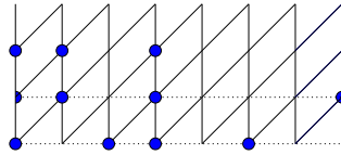
Figure 12: A DA on the cylinder. The maximum source has 4 cells, the area is 10. The right most and left most vertices are identified.
