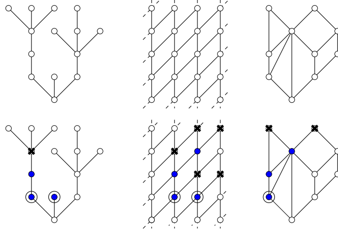
Figure 1: On the first line, three examples of agreeable graphs on which the directed edges are directed upwards. The first example is a tree, the second is the square lattice and the third a “non-layered” agreeable graph. On the second line are represented some DA on these graphs; filled points are the cells, the crosses are perimeter sites, and the surrounded points are the minimal sources of these DA.
