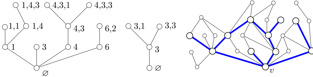
Figure 5: A representation of the tree \mathbf{t} = \{\emptyset, 1, 3, 4, 6, (1, 1), (1, 4), (4, 3), (6, 2), (1, 4, 3), (4, 3, 1), (4, 3, 3)\} . The second tree is \mathbf{t}^4 . We have \mathcal{C}_\emptyset(\mathbf{t}) = \{1, 3, 4, 6\} . On the third figure is drawn the embedding \pi_v(\mathbf{t}) on an agreeable graph, where the edges are directed upward.
