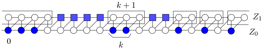
Figure 11: A block of k occupied positions in Z_0 determines k+1 empty position on Z_1 (surrounded by rectangles). The little squares figure out the uncertain cells, that can not be determined just in view of the gas occupation in Z_0 .
