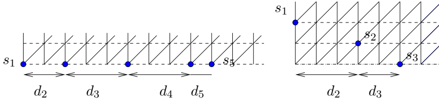
Figure 9: On the first picture, the sources considered in Proposition 3.6. The second picture illustrates the sources considered in Proposition 3.7.
