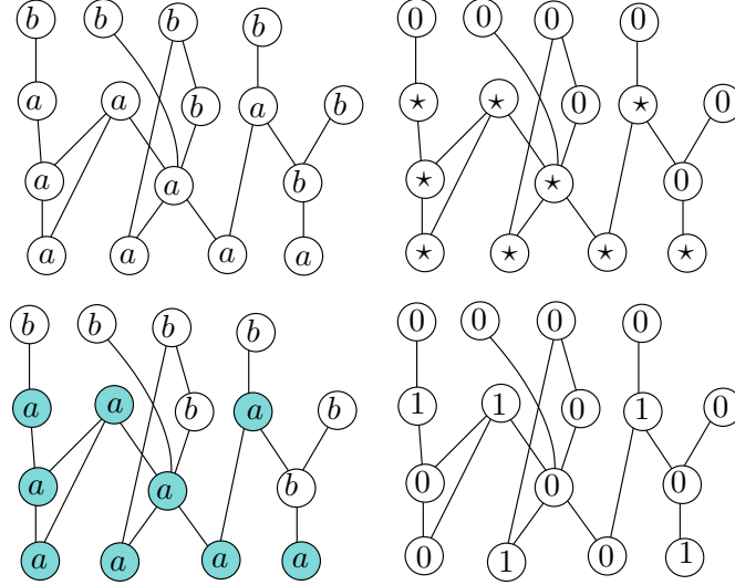
Figure 3: On the first column on top, a random coloring. Below, the family of DA derived from it. On the second column on top, the beginning of the computation of the gas occupation. “*” stands for the places where the calculus X_x \leftarrow \prod_{c: \text{children of } x} (1 - X_c) must be done. Below, the gas occupation has been computed.
