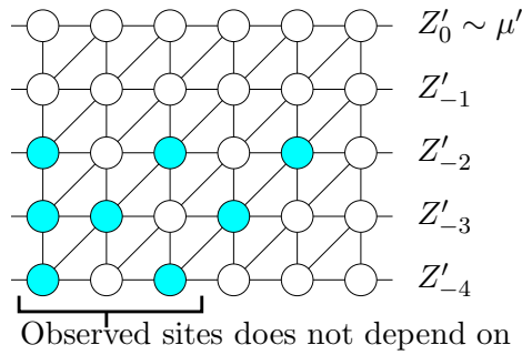
Figure 7: The colored sites are the sites where the Bernoulli( p ) coloring = 1. The gas occupation on the three first cells on the last row depends only on the DA (with these three cells as over-sources). The height of this DA is so small that the gas occupation of these cells does no depend on Z'_0 .
