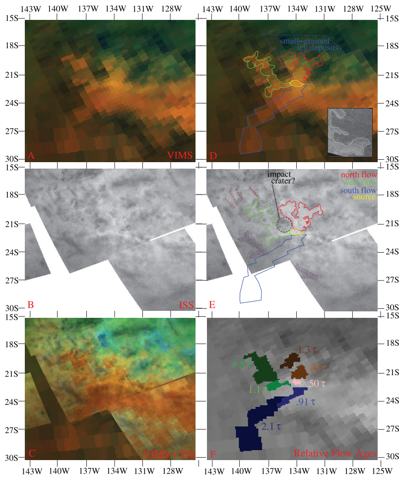
Figure 2. Cylindrical maps of western Tui Regio from (a) VIMS, (b) ISS, (c) a combination of VIMS and ISS that facilitates intercomparison, (d) annotated VIMS, and (e) ISS views, a Ta RADAR map of a different flow field at the same scale [Lopes et al. , 2005] (Figure 2d inset), and (f) the relative ages of individual flows. The VIMS mosaic was generated from observations obtained during the Ta Titan flyby on 2004 October 26 and the Tb Titan flyby on 2004 December 13. The viewing geometry (phase angle of 12^{\circ} – 14^{\circ} for Ta and 16^{\circ} – 18^{\circ} for Tb) and lighting conditions are similar enough from these two flybys to allow valid comparisons between the two. The lower-resolution data in the southwestern portion of the VIMS mosaic is from Ta and has a spatial resolution of \sim 40 km/pixel; the medium-resolution data in the remainder has a resolution of \sim 20 km/pixel, or \sim 2 pixels/degree. At 25^{\circ} S, each degree corresponds to 45 km in latitude and 41 km in longitude. Colors are the same as in Figure 1 but the image has been contrast-enhanced. The ISS view is a mosaic generated from images taken during the Tb flyby and has a plate scale of 2 km/pixel. We estimate the absolute location error of the map to be 1–3 degrees. The annotated VIMS and ISS maps illustrate our interpretations as described in the text. The relative ages of lava flows in terms of the unknown weathering timescale \tau are shown in Figure 2f, along with the areas to which the ages correspond, on top of a VIMS 5 micron map.
