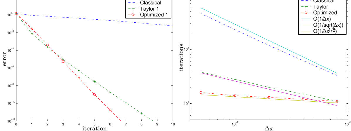
Figure 8: Left: convergence factor comparison for the eight subdomain case. Right: Asymptotic behavior as the mesh is refined with an overlap L = \Delta x for the eight subdomain case, with \Delta t = O(\Delta x) , together with the predicted rates from the two subdomain analysis.
