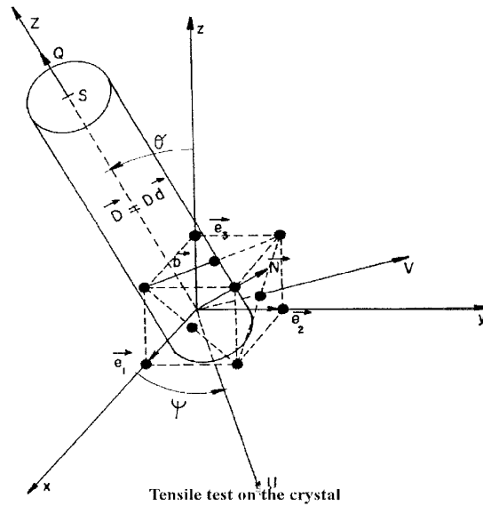
Fig. 4. Geometrical representation of a tensile test on the crystal.
