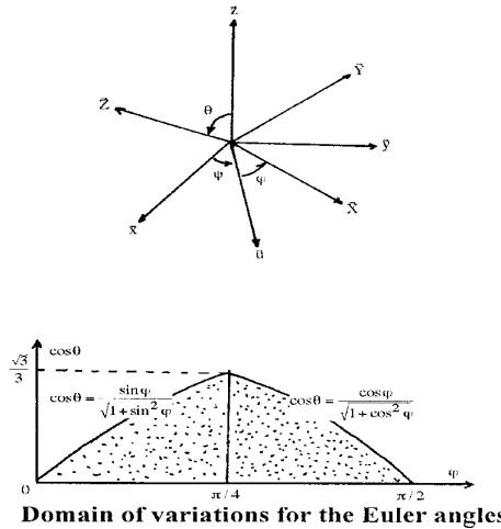
Fig. 6. Limits on the angles for the isotropic polycrystal.
