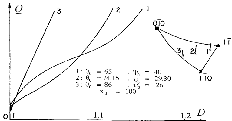
Fig. 5. Global tensile responses with the orientation of the crystal.
