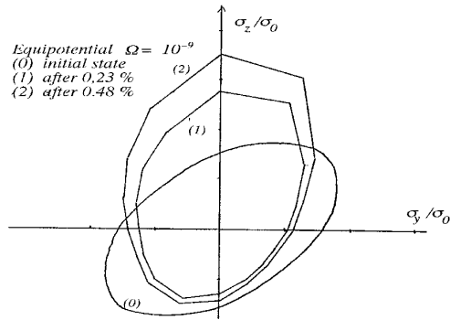
Fig. 14. Viscoplastic potential surface with the axial strain.
