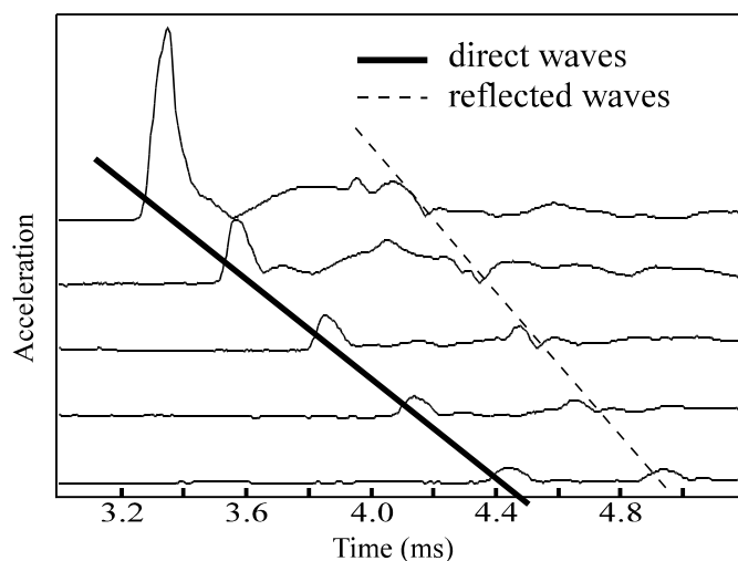
Figure 7 : Acceleration measurements (magnitude) for mid-depth sensors showing direct and reflected waves (drop-ball test).
