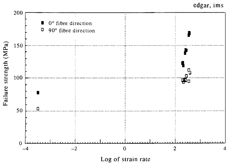
Fig. 4. Failure strength versus strain rates.
