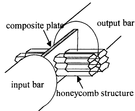
Fig. 1. Detail of the experimental device.
