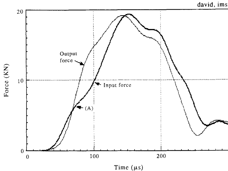
Fig. 5. Input and output forces.
