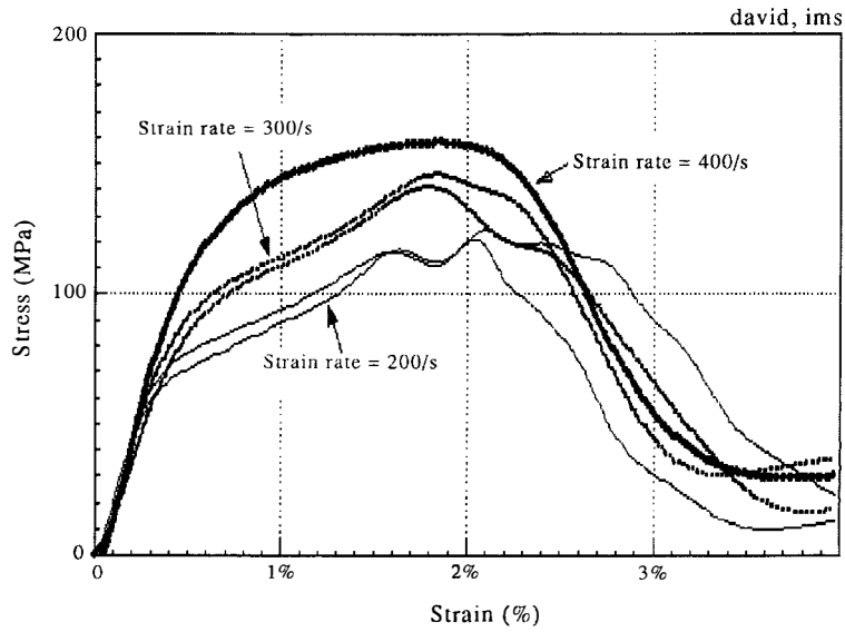
Fig. 3. Influence of strain rates.
