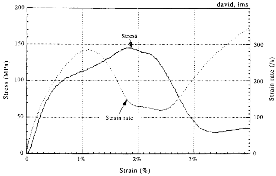
Fig. 2. Stress and strain rate versus strain.
