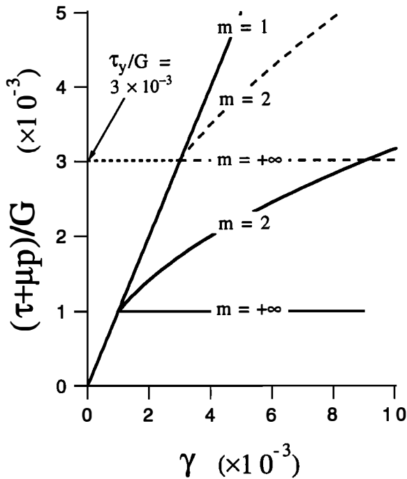
Figure 2. The uniaxial stress-strain curve of the overburden material is linear for an equivalent stress less than the yield stress \tau_y , which has for value either G \times 10^{-3} (solid curves) or 3G \times 10^{-3} (dashed curves). This relation becomes a power law with exponent m if the initial yield stress is exceeded. The two values for m of 1 and +\infty corresponds to an elastic and an elastic, perfectly plastic response, respectively.
