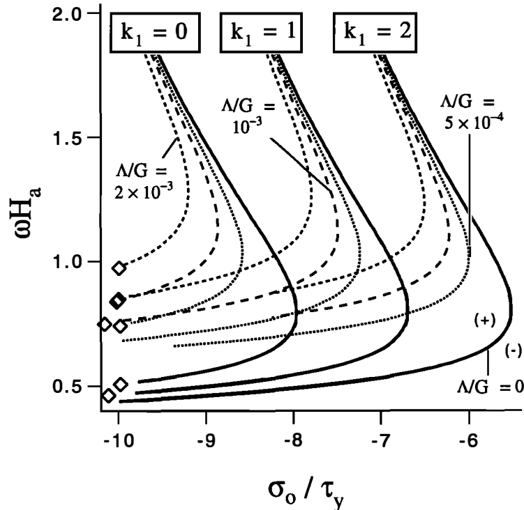
Figure 9. Influence of the stress gradient parameter k_1 . Curves of similar type (solid, dotted, or dashed) correspond to the same stability exponent. The finite element results are obtained for deformation theory and for \Delta\rho g H_a / G = 1.41 \times 10^{-3} corresponding to an overburden thickness of 2 km. The substratum thickness is 1 km, and the boundary condition at the basement is one of slip with no friction. The diamonds, which indicate loss of ellipticity, are not shown for k_1 = 2 .
