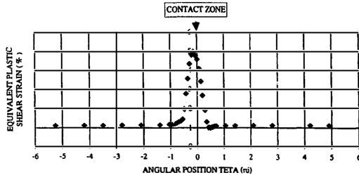
Fig. 8. The maximal plastic shear strain \epsilon_{max}^z versus \theta (rad), F = 10 N, \mu = 0.5 (plastic shakedown state).
