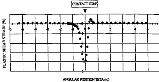
Fig. 7. Distribution of the plastic shear strain \epsilon_p^z versus \theta (rad), F = 10 N, \mu = 0.5 (plastic shakedown state).
