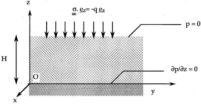
Figure 1. Layer subjected to a uniform overload.
