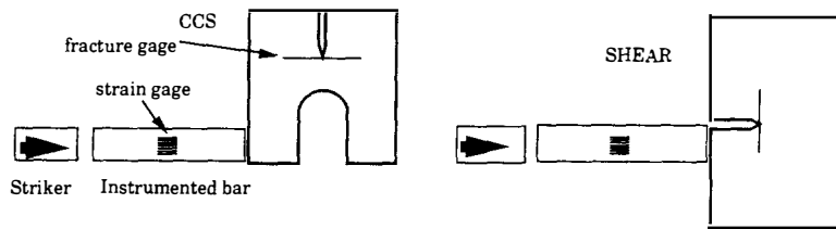
Figure 1: Experimental setup
