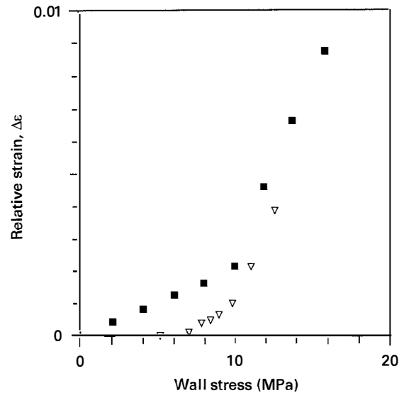
Figure 26 The relative variation of strain \Delta\epsilon versus real wall stress. Comparison between (▽) experimental data and (■) numerical simulation.
