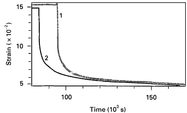
Figure 9 Measured geometrical recovery over 24 h.
