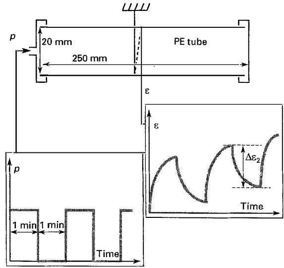
Figure 24 The EAHF experiment.
