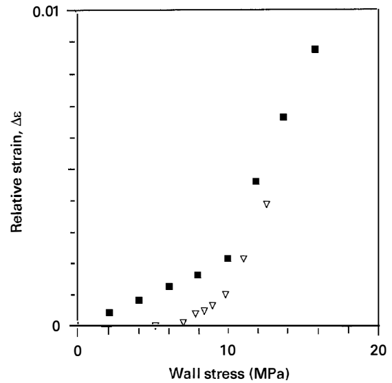
Figure 26 The relative variation of strain \Delta\epsilon versus real wall stress. Comparison between ( \nabla ) experimental data and ( \blacksquare ) numerical simulation.
