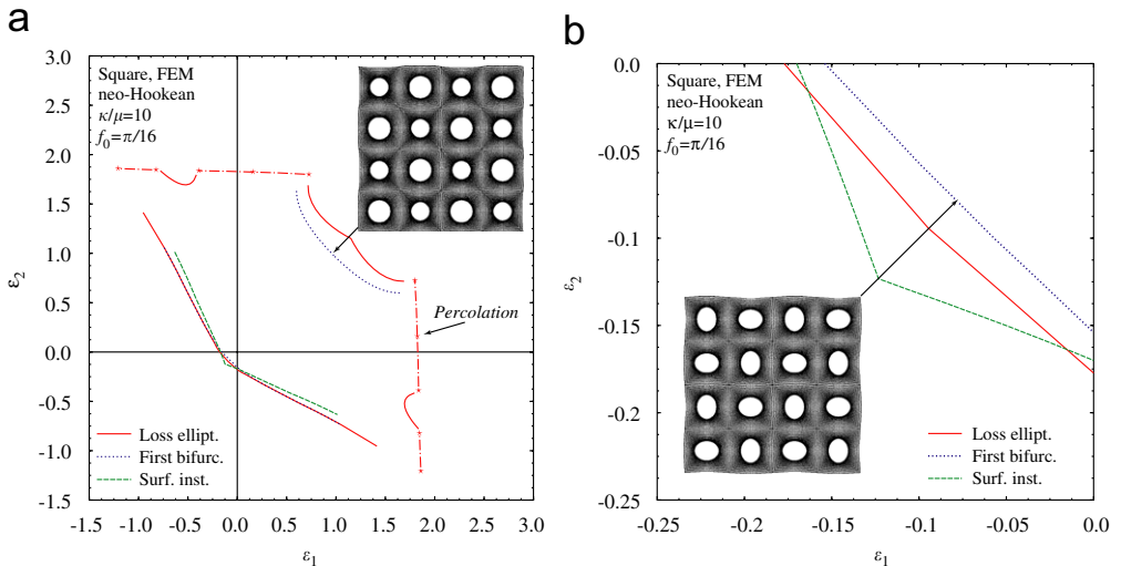
Fig. 4. In (a) are plotted in principal logarithmic strain space the microscopic (dotted lines) and macroscopic (solid lines) onset-of-failure curves of a neo-Hookean matrix elastomer with square microgeometry. The macroscopic strains corresponding to the onset of an instability at the free surface of the voids (dashed lines) and to percolation (dashed–dotted–starred lines) are also recorded. A blow-up of the biaxial compression region in (a) is plotted in (b). The eigenmodes corresponding to the first bifurcation encountered under plane strain equibiaxial tension and compression ( \varepsilon_1 = \varepsilon_2 \leq 0 ) are also depicted.
