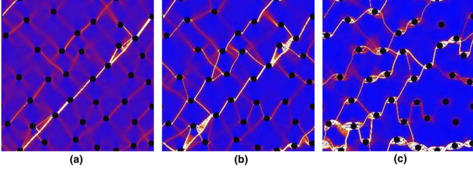
Fig. 10. Snapshot of the local equivalent strain for type-B loading and different triaxiality ratios: (a) \tau = \frac{1}{3} ; (b) \tau = 1 and (c) \tau = 3 .
