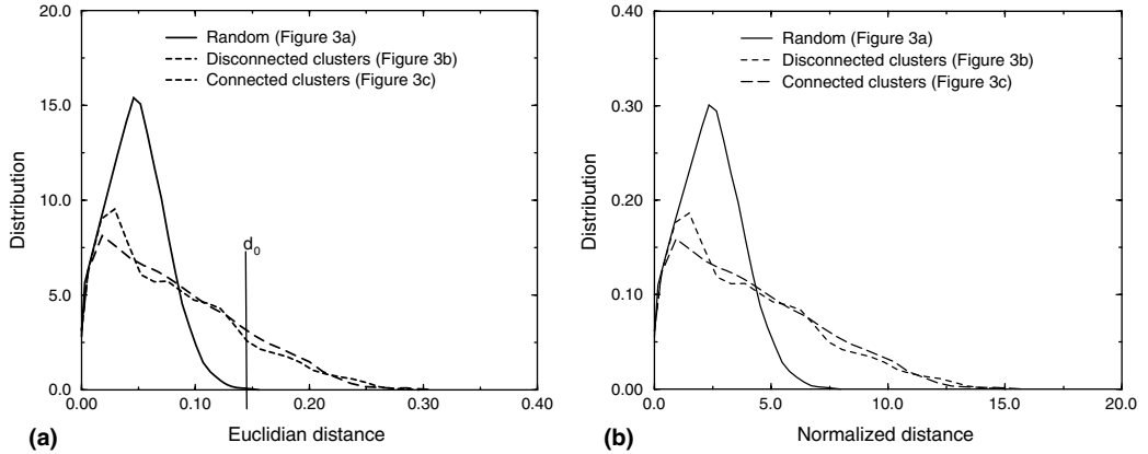
Fig. 16. Two-dimensional microstructures with single pore size: (a) distribution of the distance function and (b) distribution of the normalized distance function.
