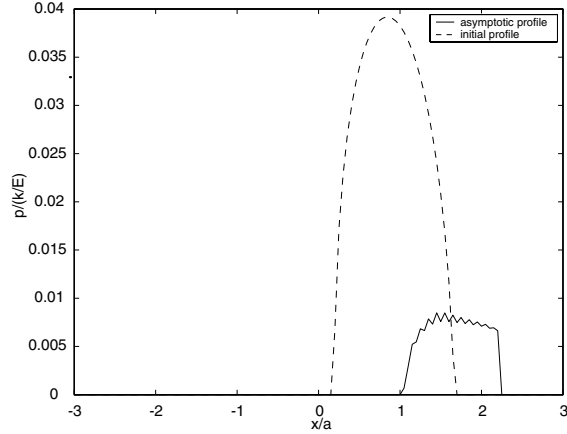
Fig. 11. Stabilized contact pressures at t/T = 0.25 .
