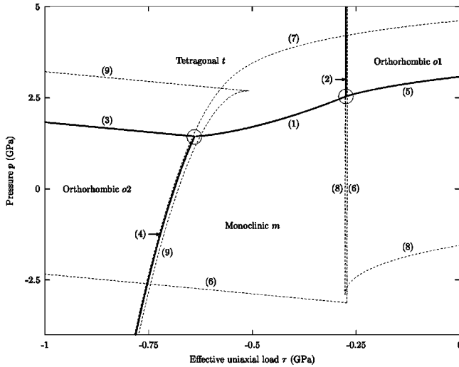
FIG. 4. Calculated phase diagram of zirconia in the (\tau, p) plane at room temperature. Same legend as in Fig. 2.
