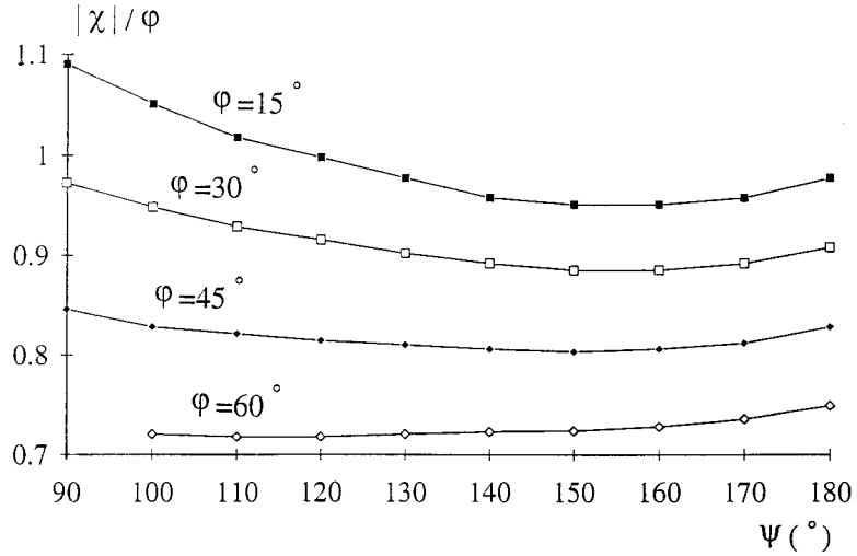
Figure 4. Figure 4. The ratio |\chi|/\phi as a function of the angle \psi , for various values of the angle \phi .
