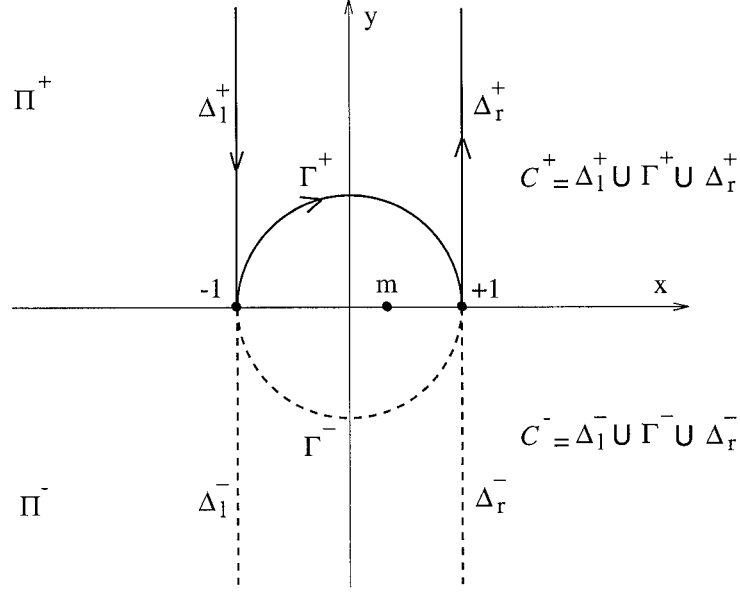
Figure 2. Integration paths in the z -plane.
