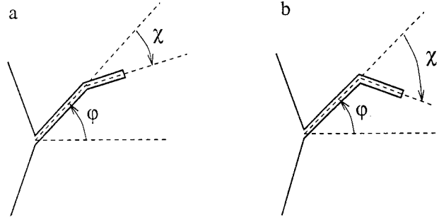
Figure 3. Figure 3. The two possible situations after the kink: |\chi| < \phi (a); |\chi| > \phi (b).
