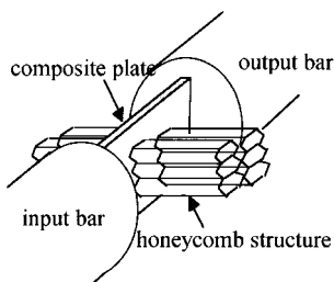
Fig. 4. Detail of the experimental anti-buckling device.
