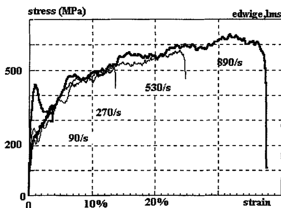
Figure 6. Stress-strain curves at various strain-rates.
