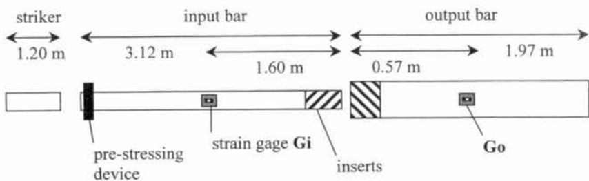
Figure 2. Scheme of the complete set-up.
