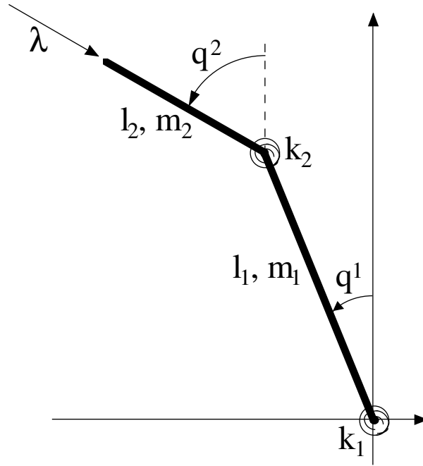
Fig. 1. Geometry of the double pendulum.
