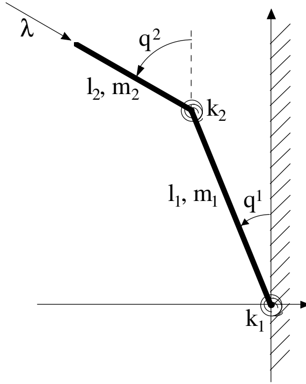
Fig. 3. Double pendulum with obstacle.
