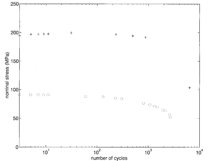
Figure 9 Load versus number of cycles for a LCF test on SiMo SG cast iron at 600°C (+) and 700°C (o) ( \Delta\epsilon = \pm 0,25\% ).
