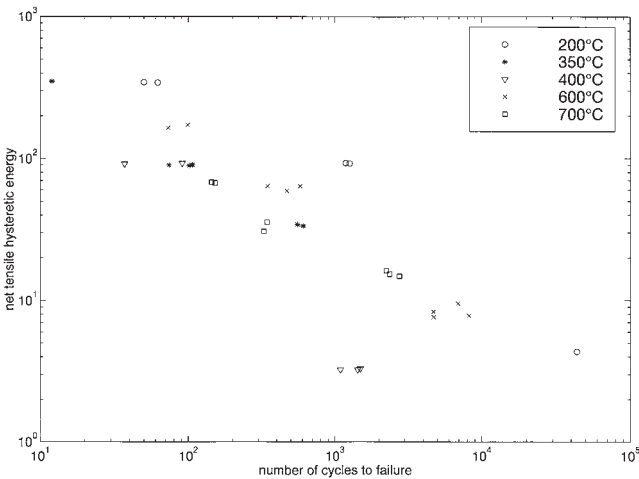
Figure 8 Net tensile hysteretic energy obtained with LCF tests results on SiMo SG cast iron with the test conditions corresponding to Table 2. All values are in J/mm 3 .
