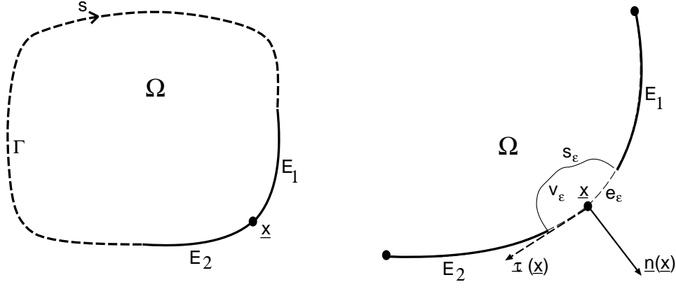
Figure 2. Boundary partitioning
