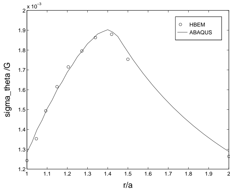
Figure 6. Example 2 (hypersingular and shortcut): hoop stress
