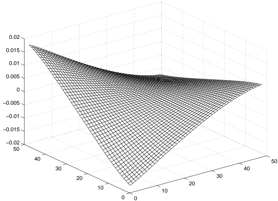
Figure 4: Example 2: variation of J(x_i, 1) (horizontal units refer to a regular 50 \times 50 grid used for the plot).
