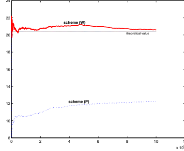
Figure 4: n \mapsto \bar{\nu}_n(\phi) , \alpha = 5/3
