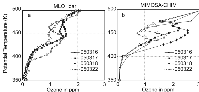
Figure 4. (a) Two-hour integrated ozone profiles measured by the MLO lidar on the nights of 16, 17, 18, and 22 March 2005. (b) MIMOSA-CHIM ozone profiles modeled at 0600 UT on the same nights and location as that measured by lidar.
