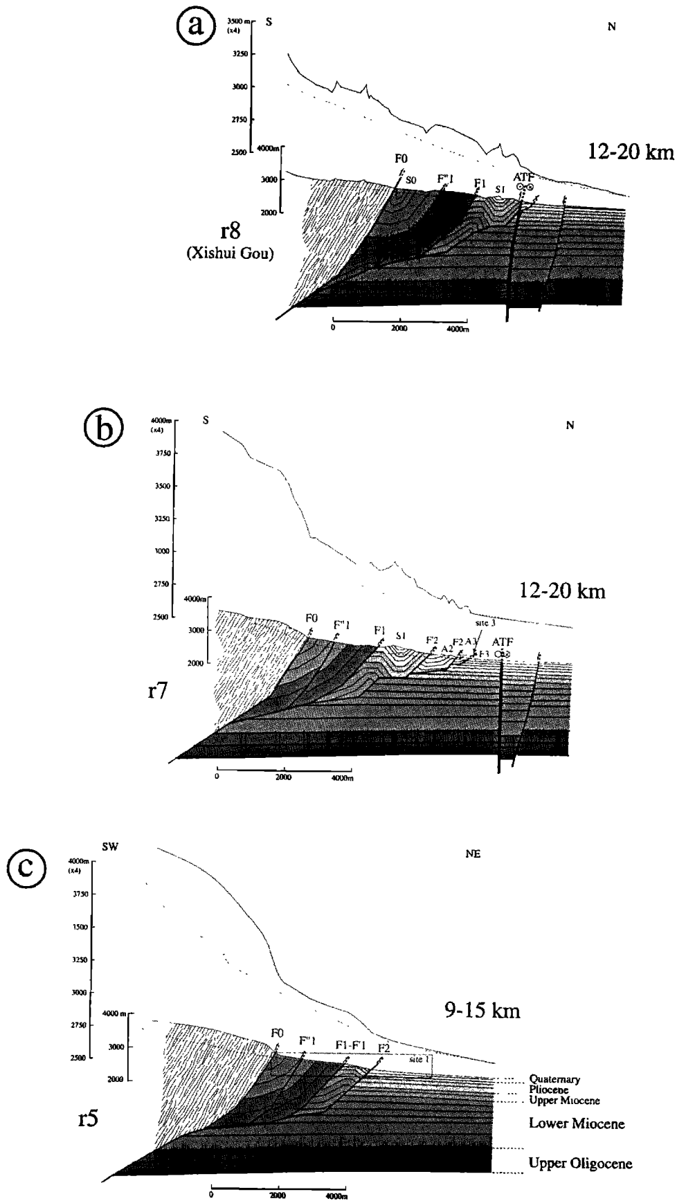
Figure 7. Plausible retrodeformable cross sections across thrust wedge, accounting for field observations (a) along stream r8 (Xishui Gou), (b) along r7, and (c) along r5. Cumulative shortening deduced from balancing of sections is indicated. Topographic profiles of streams and adjacent relief are shown with vertical exaggeration of 4.
