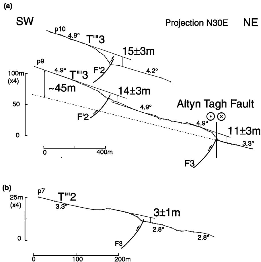
Figure 13. (a) Projection N30°E of profiles p10 and p9 across F2 and F3 and vertical throw across different thrusts. (b) Profile p7 across F3 on T'''2.
