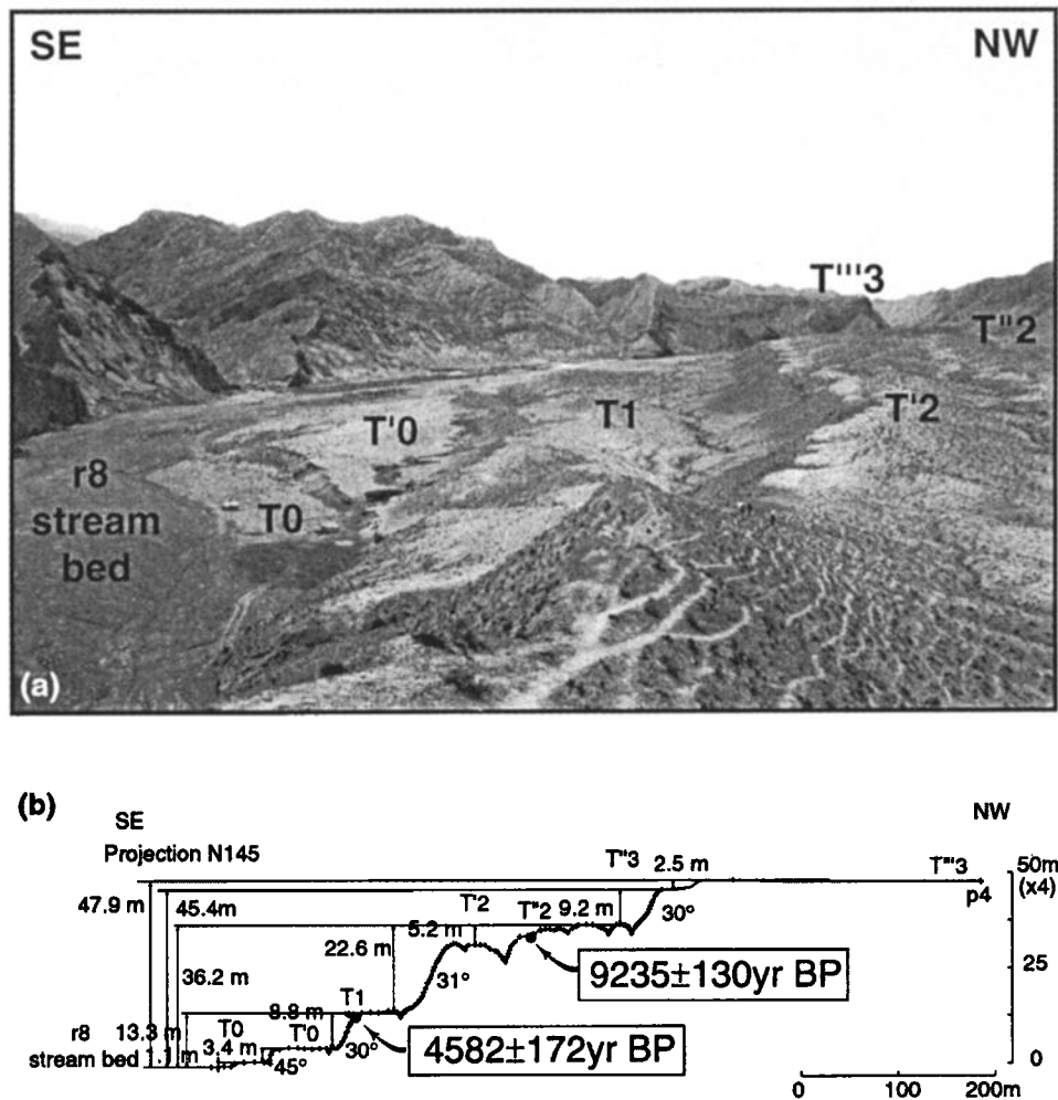
Figure 11. (a) View, to the west, at site 2, of abandoned terrace flight above entrenched streambed r8. (b) Profile p4 across terraces and relative heights.
