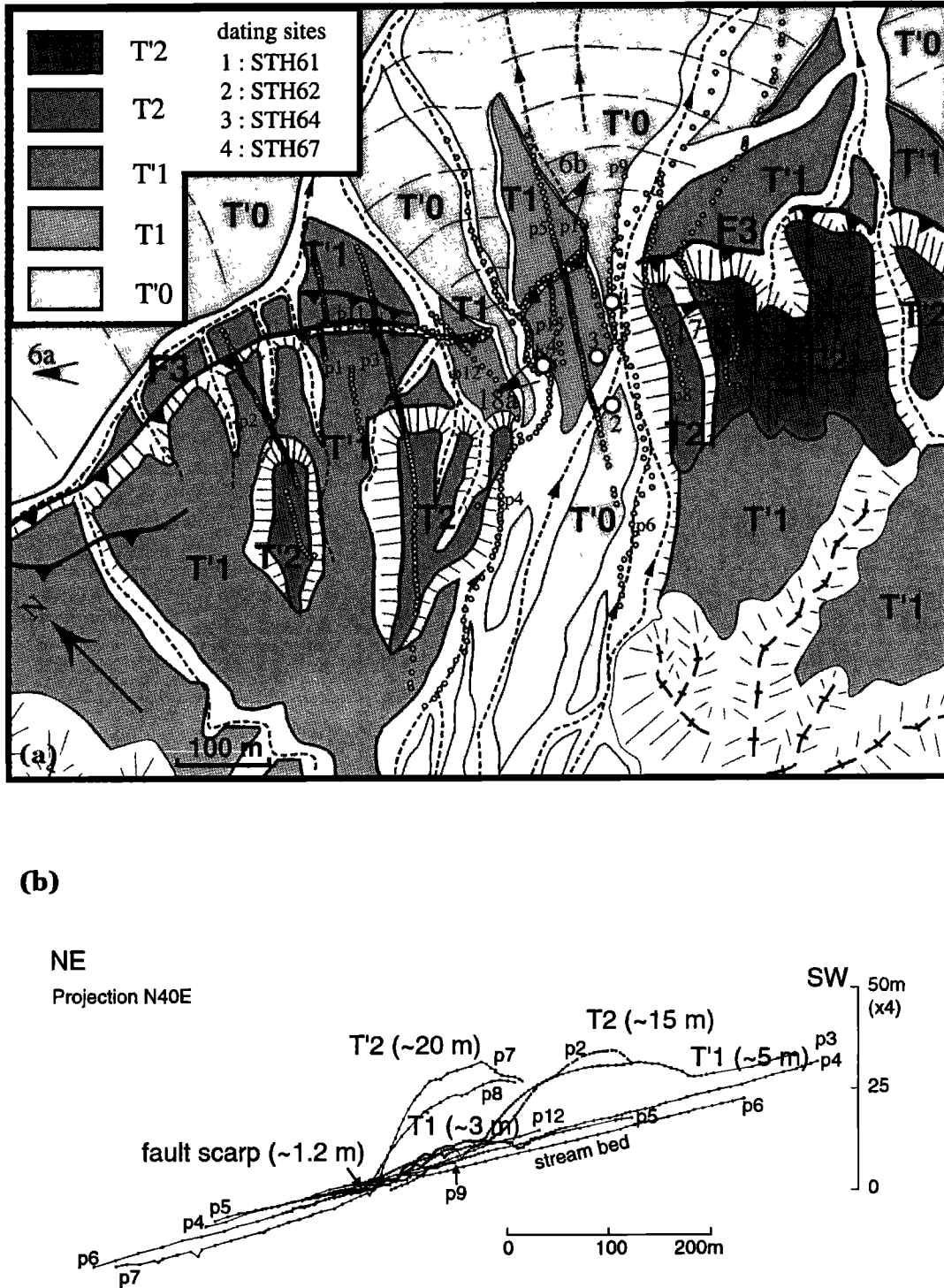
Figure 14. (a) Geomorphic map of site 3. Hills correspond to anticline A3. Note scarps of thrust F3 that bound A3 to the northeast. Small dots are levelling points of topographic profiles. Large dots refer to sampling sites for radiocarbon dating. (b) Projection of topographic profiles across anticline A3 at site 3.
