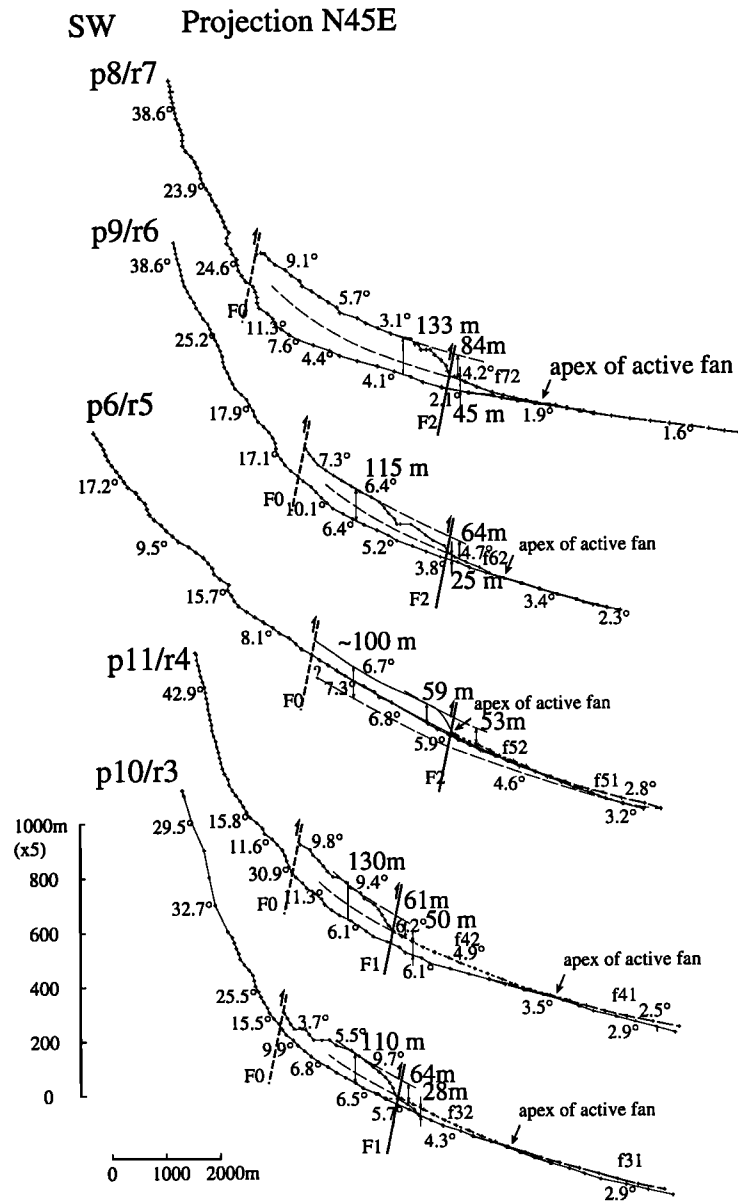
Figure 22. Projection of streams, terrace T3, and fan profiles.
