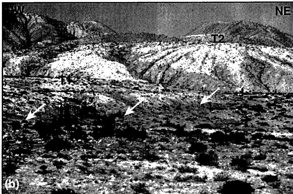
Figure 6. (a) View, to the south, of anticline A3, foremost growing fold above southwest dipping thrust ramp (F3). Larger flexure in the background is capped by terrace T3. (b) Scarp, 1 to 2 m high, of thrust F3, due to recent earthquake, offsets young terrace T1. Note rounded, eroded riser of T2 and deeply incised gullies.
