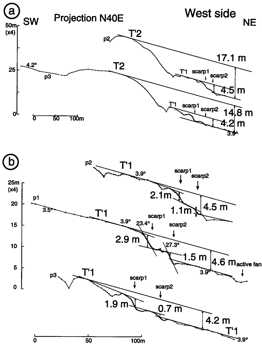
Figure 16. (a) Topographic profiles on T2 west of the stream. (b) Topographic profiles on T'1 and across F3 scarp.
