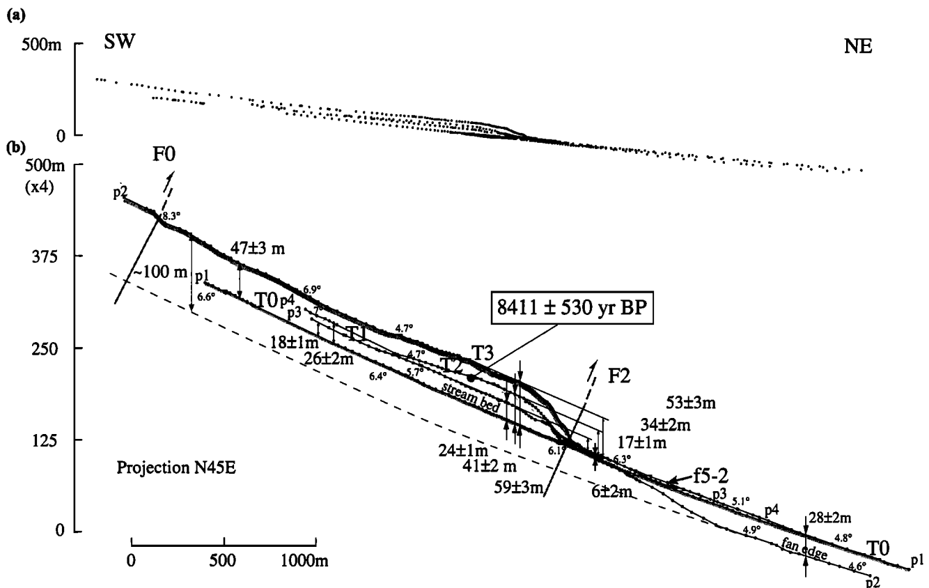
Figure 9. Projection N45°E of profiles at site 1: (a) 1×1 scale; (b) projection with vertical exaggeration (×4). Slopes and heights of terraces above streambed and footwall are indicated. Plausible total offset of T3 inferred from fan slope variation in piedmont may reach ~100 m (see text).
