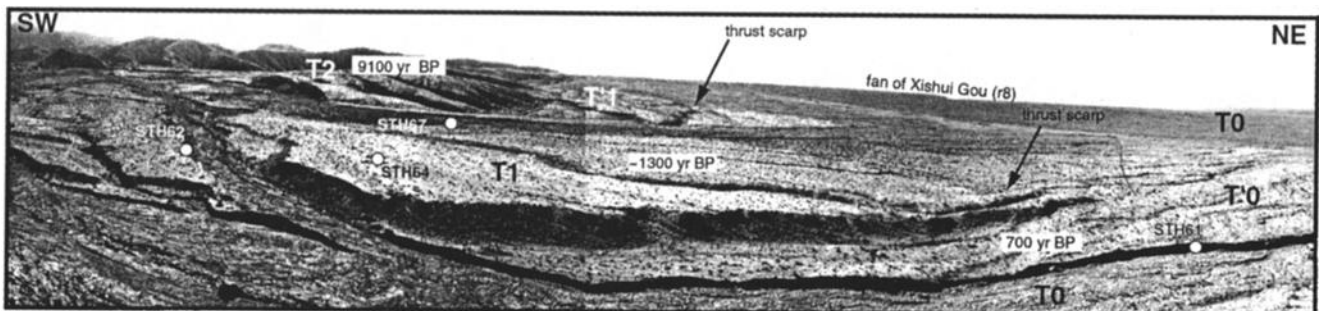
Figure 17. View to the northwest of folded and faulted lower terraces (T'0 and T1) at site 3. Ages of terrace abandonment deduced from radiometric dating are indicated (see text).
