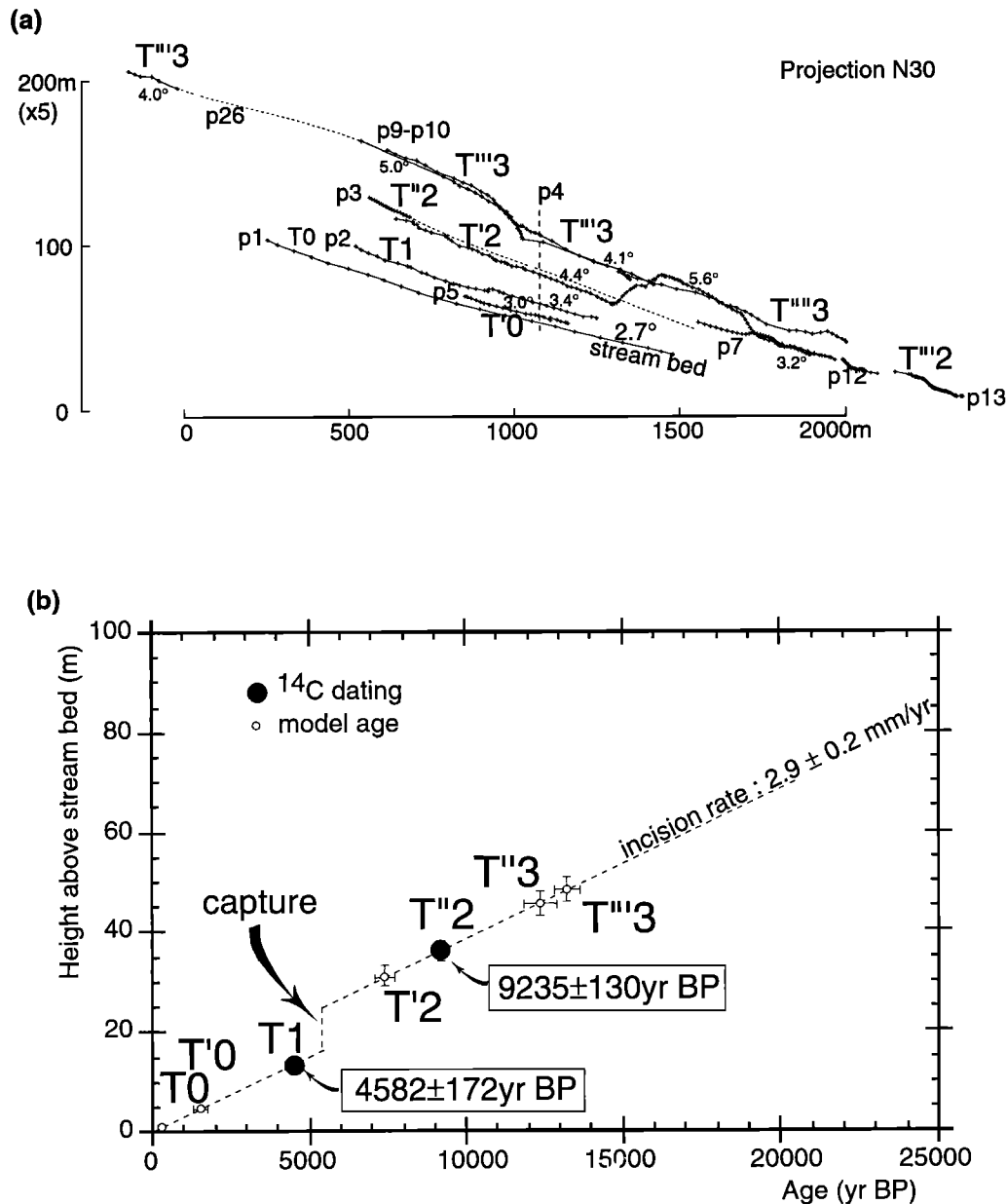
Figure 12. (a) Topographic profiles projected N30°E at site 2. (b) Age of terraces, inferred from incision rate assumed to be constant and two dated terraces (T1 and T'2).
