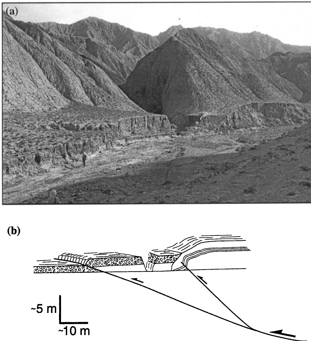
Figure 5. (a) Seismic scarp across a recent terrace of stream r7, ~200 m southwest of F2. Southwest view is of scarp (black arrows) across terrace and fold (white arrow) with clear overturned alluvial layers unconformably covered by more recent terrace deposits. (b) Schematic interpretation of scarp and fold geometry associated with thrust propagation.
