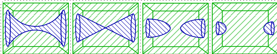
Fig. 17: Sliced view of the growing of the two possible domains in case 2 \leq k_\lambda \leq 2n - 2 .
