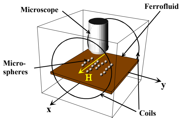
Figure 5. Schematic experimental set-up.
