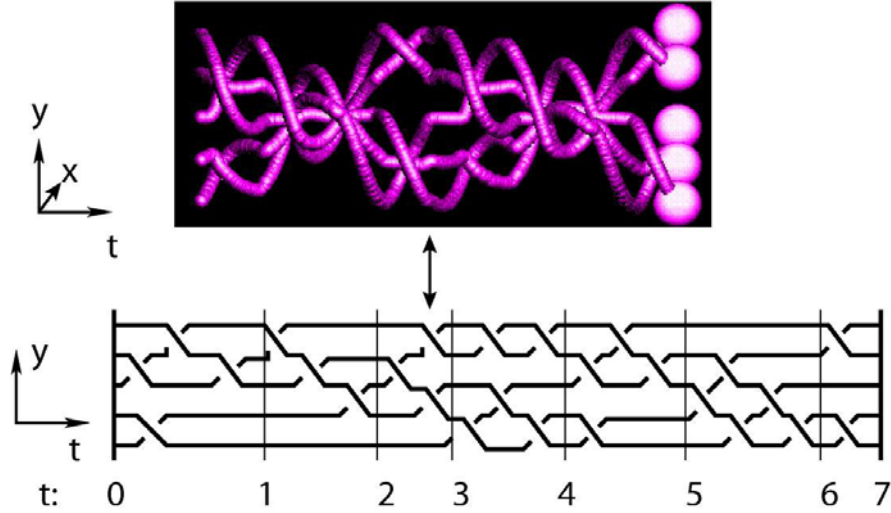
Figure 8. The two-dimensional motion of 5 microspheres is extended to three-dimensional space-time with the trace of each particle in time (upper). Projecting onto (y,t) -axis gives the braid for the motion (lower).
