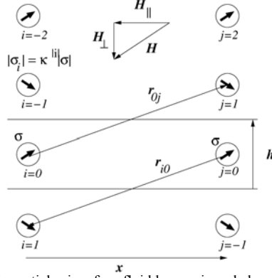
Figure 11. Pair of non magnetic particles in a ferrofluid layer, viewed along the confinement plates, and the series of dipole images accounting for the boundary conditions of the magnetic field along the plates.
