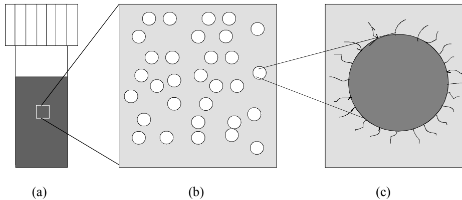
Figure 1. Schematic picture of ferrofluid on three length scales: a: On a macroscopic length scale, it resembles an ordinary liquid with a uniform magnetization. b: On a colloidal length scale, solid nanoparticles dispersed in a liquid. c: Each particle consists of a single domain magnetic core, e.g. iron oxide, and a surface grafted with polymer chains, particle size \sim 10 nm.
