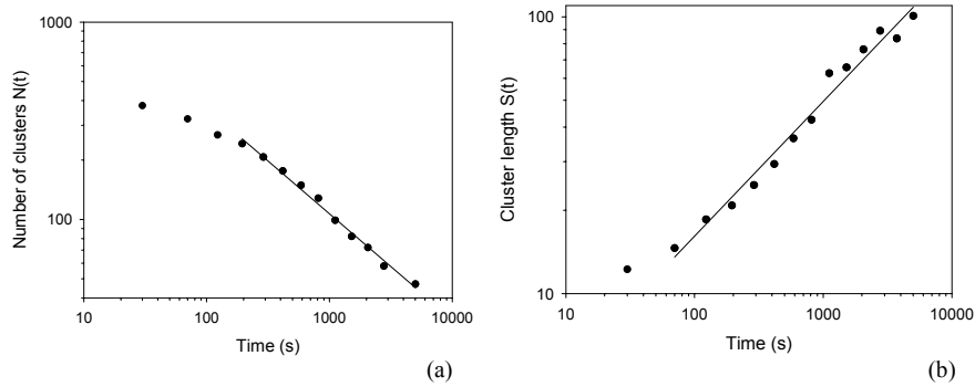
Figure 7. (a) The number of clusters and (b) cluster length versus time for aggregation of 10 \mu\text{m} spheres in a 10 Oe magnetic field. The solid lines are fits to a power law with exponents (a) z' = 0.53 and (b) z = 0.50 .
