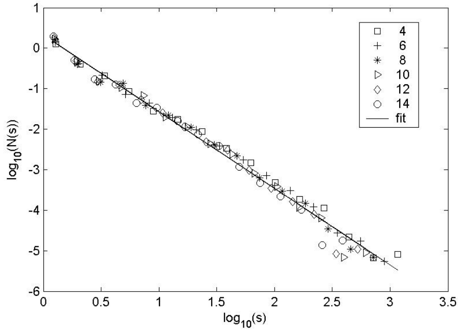
Figure 3: The distribution N(s) for different clip levels averaged over all eight experiments. The numbers inserted in the figure are the clip levels C . The solid line is a linear fitting to the data points and has a slope -1.89 .
