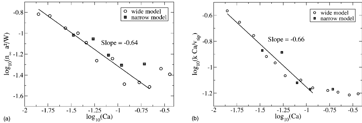
FIG. 9. Double logarithmic plots of (a) the saturated mass density n_{\infty} and (b) of the speed of the most advanced finger, v_{\text{tip}} , as a function of the capillary number, for the two sets of experiments. Both plots are consistent with a scaling in the form n_{\infty} \propto \text{Ca}/v_{\text{tip}} \propto \text{Ca}^{-\alpha} , with \alpha \approx 0.65 .
