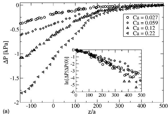
FIG. 7. Plot of the pressure difference \Delta P(z) = P(z) - P(\infty) measured by the pressure sensor located in the position (x_s, z'_s) = (38 \text{ mm}, 280 \text{ mm}) . The inset is the same data plotted in a semilogarithmic plot where P(z) is scaled with \Delta P(0) = P(z=0) - P(\infty) to illustrate the decay of the pressure field. (a) is for the wide model and (b) is for the narrow model.
