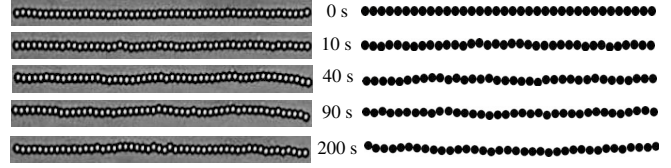
FIG. 1. Typical dynamic roughening of dipolar chains of 52 magnetic holes of diameter 4 \mu\text{m} after a sudden decrease of the external magnetic field: experiments (left) and simulations (right).
