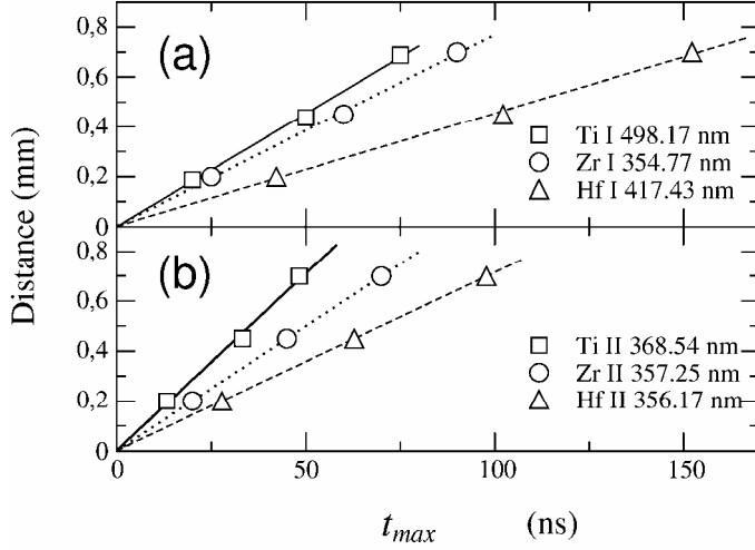
Figure 11 : Distance from target as a function of t_{max} for ablation of Ti, Zr and Hf in 500 Pa He with F_{las} = 3.0 \text{ Jcm}^{-2} ( \lambda_{las} = 800 \text{ nm} ). The slopes represent the most probable velocities of neutral atoms (a) and ions (b).
