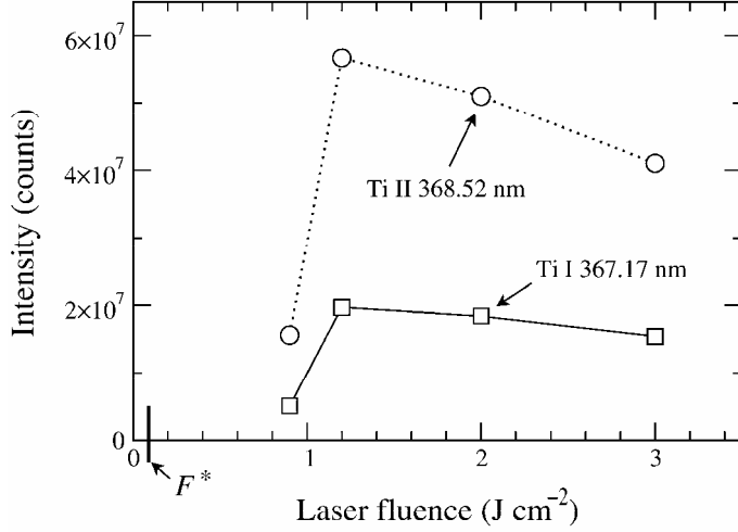
Figure 13 : Spectral line emission intensities of ions and neutral atoms as a function of F_{las} for Ti ablation in 500 Pa He at \lambda_{las} = 800 nm.
