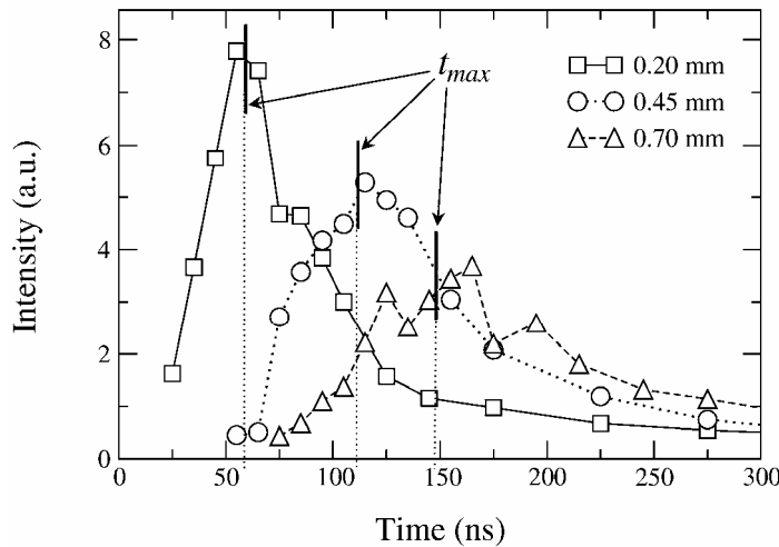
Figure 9 : Emission intensity of the Hf I 417.43 nm spectral line as a function of time for different distances from target. The recordings correspond to ablation of Hf in 500 Pa He with F_{las} = 3.0 \text{ Jcm}^{-2} ( \lambda_{las} = 800 \text{ nm} ).
