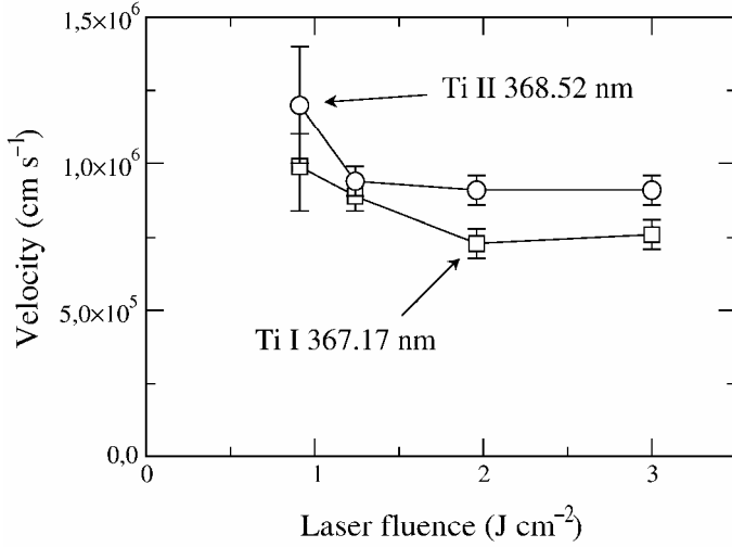
Figure 12 : Propagation velocities of neutral atoms and ions as a function of F_{las} observed during Ti ablation in 500 Pa He using \lambda_{las} = 800 \text{ nm} .
