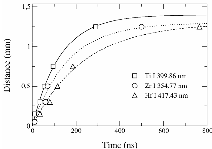
Figure 10 : Distance from target as a function of t_{max} for ablation of Ti, Zr and Hf in 500 Pa He with F_{las} = 3.0 \text{ Jcm}^{-2} ( \lambda_{las} = 800 \text{ nm} ).
