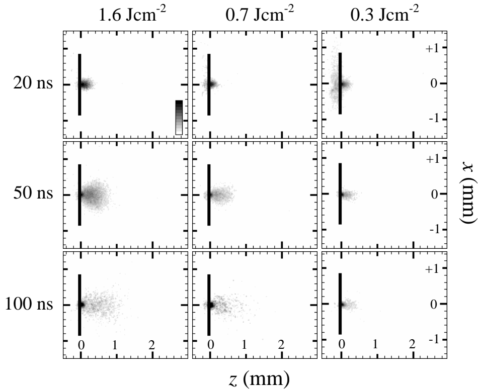
Figure 2 : Plasma images recorded for different laser fluences and time delays during Ti ablation in 500 Pa He using the second harmonic ( \lambda = 400 nm). Colour scaling is adjusted for every image to the maximum intensity.
