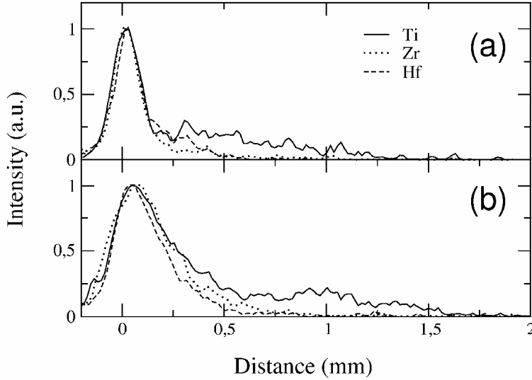
Figure 7 : Intensity profiles recorded during ablation of Ti, Zr and Hf for t = 100 (a) and 900 ns (b) in 500 Pa He with F_{las} = 1.6 Jcm -2 and \lambda_{las} = 400 nm.
