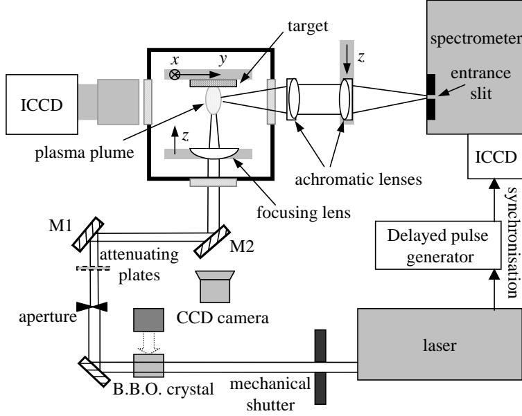
Figure 1: Experimental set-up. Mirrors M1 and M2 with coatings for reflection at 45° incidence at \lambda_{las} (800 or 400 nm) were used.
