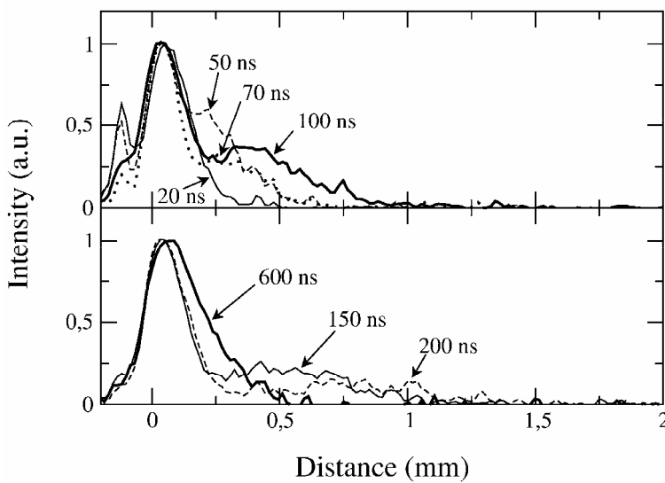
Figure 5 : Intensity profiles recorded for ablation of Ti in vacuum. The other experimental conditions are identical to those of figure 3.
