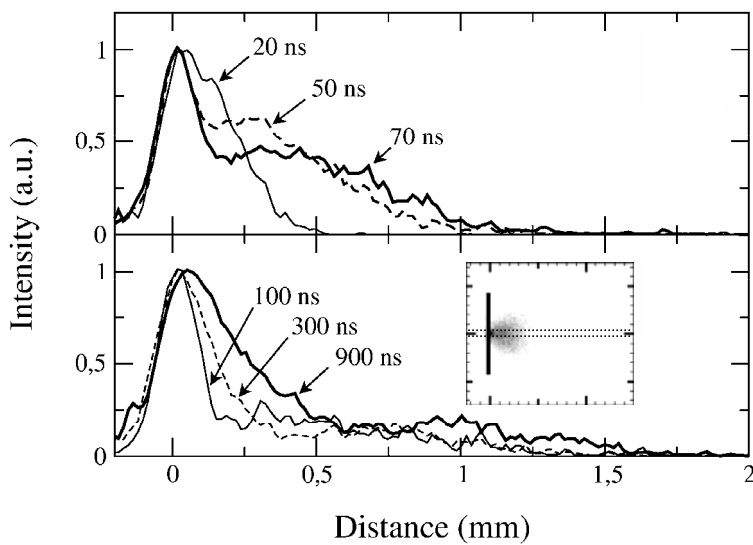
Figure 3 : Intensity as a function distance from target for different times and F_{las} = 1.6 Jcm -2 . The other experimental conditions are identical to those of figure 2.
