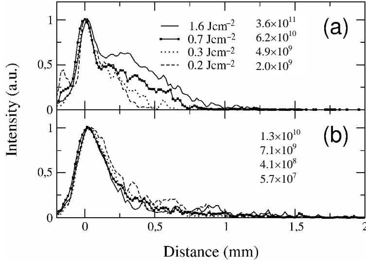
Figure 6 : Intensity profiles recorded for different laser fluences for t = 20 (a) and 400 ns (b) during ablation of Ti in 500 Pa He with \lambda_{las} = 400 nm.
