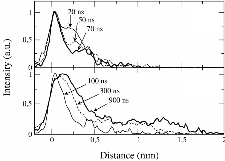
Figure 4 : Intensity profiles recorded during ablation of Ti in 500 Pa He with F_{las} = 3 \text{ Jcm}^{-2} using the fundamental wavelength at \lambda = 800 \text{ nm} .
