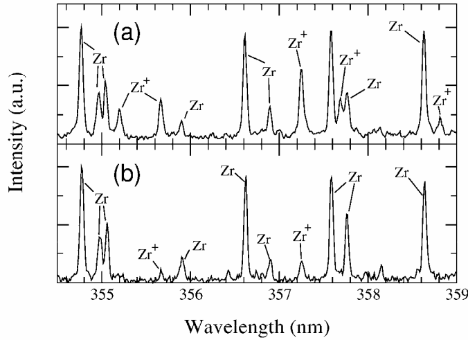
Figure 8 : Optical emission spectra recorded during ablation of Zr in 500 Pa He with F_{las} = 3.0 \text{ Jcm}^{-2} ( \lambda_{las} = 800 \text{ nm} ) for t = 50 (a) and 70 \text{ ns} (b) and z = 150 \mu\text{m} .
