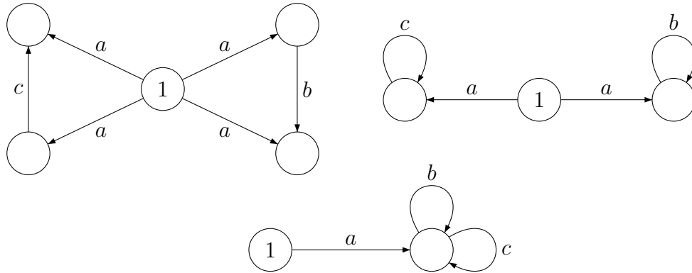
Figure 1: Computing the representation of H = \langle aba^{-1}, aca^{-1} \rangle
