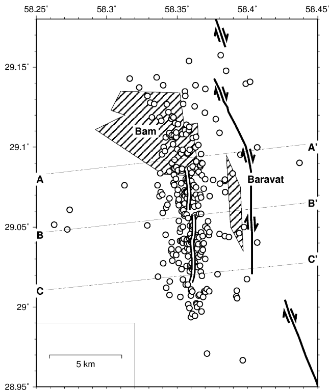
Figure 6. Selected seismicity of the 331 earthquakes located with a rms less than 0.1 s, and uncertainties in location less than 1 km in more than 10 stations. Symbols as in Fig. 4.
