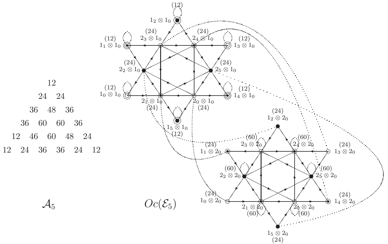
Figure 4: Dimension d_n and d_x of the blocks for \mathcal{E}_5 .
