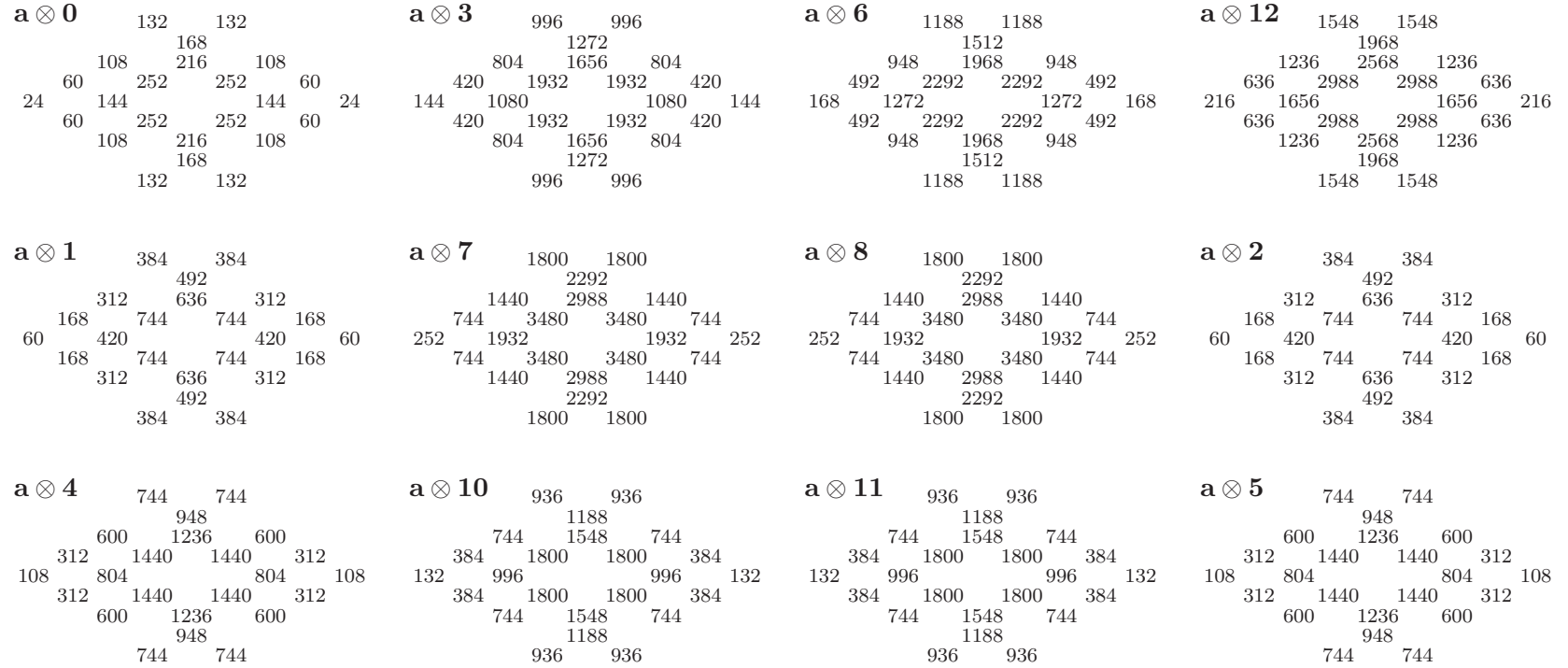
Figure 9: Dimensions d_x for blocks labelled by Oc(\mathcal{E}_{21}) .
