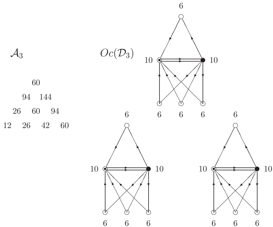
Figure 2: Dimension d_n and d_x of the blocks for \mathcal{D}_3 .
