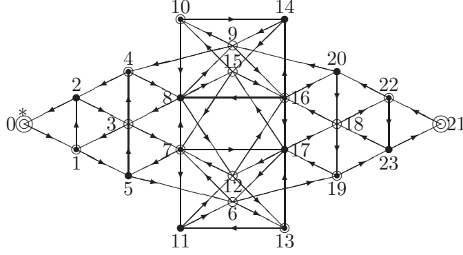
Figure 7: The \mathcal{E}_{21} graph and \mathcal{E}_{21} \leftarrow \mathcal{A}_{21} induction rules (for vertices \in J ).
