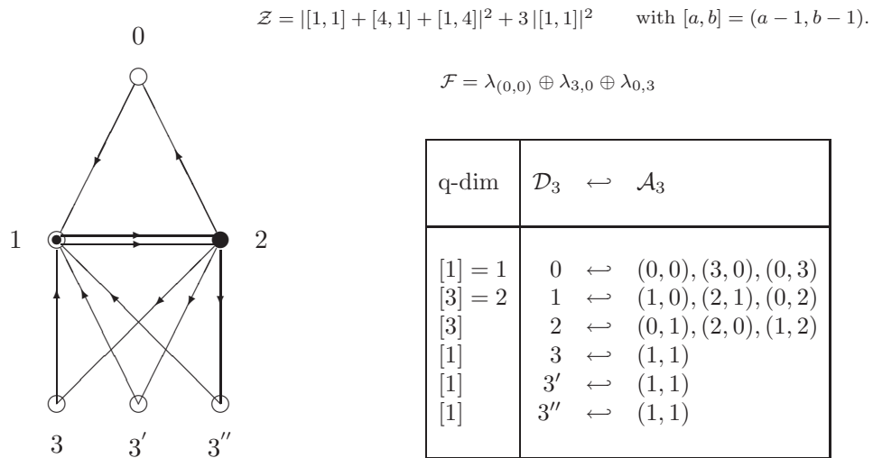
Figure 1: The \mathcal{D}_3 graph, quantum dimensions and \mathcal{D}_3 \leftrightarrow \mathcal{A}_3 induction rules.
