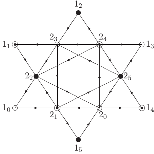
Figure 3: The \mathcal{E}_5 graph, quantum dimensions and \mathcal{E}_5 \leftrightarrow \mathcal{A}_5 induction rules.
