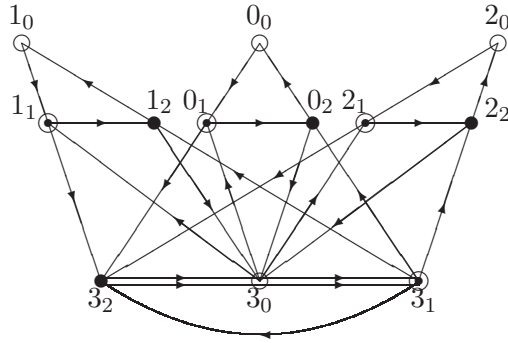
Figure 5: The \mathcal{E}_9 graph, quantum dimensions and \mathcal{E}_9 \leftrightarrow \mathcal{A}_9 induction rules.
