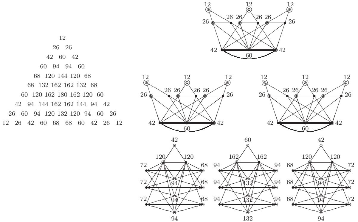
Figure 6: Dimensions d_n and d_x for the \mathcal{E}_9 graph.
