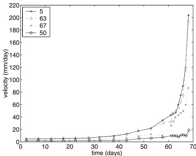
Figure 2. Velocity measurements for the four benchmark marks of the Vaiont landslide. Bench marks 5 and 63 exhibit similar acceleration. Bench mark 50 shows only a relatively small acceleration in absolute values at the end of the 60-day accelerating phase. Its acceleration is, however, significant in relative values, as seen in Figure 4. Data are from Muller [1964]. See color version of this figure in the HTML.
