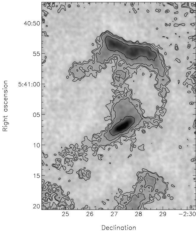
Figure 2. SCUBA 850- \mu\text{m} image of the Horsehead nebula. The region shown is approximately the same as that in Fig. 1. West is towards the top, north is to the left-hand side. Contour levels are at 2, 3, 5 and 10\sigma , where 1\sigma is 17 \text{ mJy beam}^{-1} . The FWHM beam size is 15 arcsec. The familiar Horsehead shape can be seen in this image, as well as the source SMM1 associated with the PDR along the ‘top’ of the horse’s head, and the source SMM2 in the horse’s ‘throat’.
