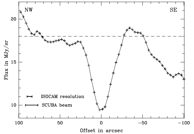
Figure 5. One-dimensional cut of the 6.75- \mu\text{m} map shown in Fig. 4 through the central position of SMM2, orthogonal to its long axis. The x -axis is marked in arcsec offset from SMM2, with the north-westerly direction marked as positive. The y -axis is labelled in units of \text{MJy sr}^{-1} . A clear absorption trough can be seen at the position of SMM2. The horizontal dashed line is a fit to the extended emission of the cloud away from SMM2.
