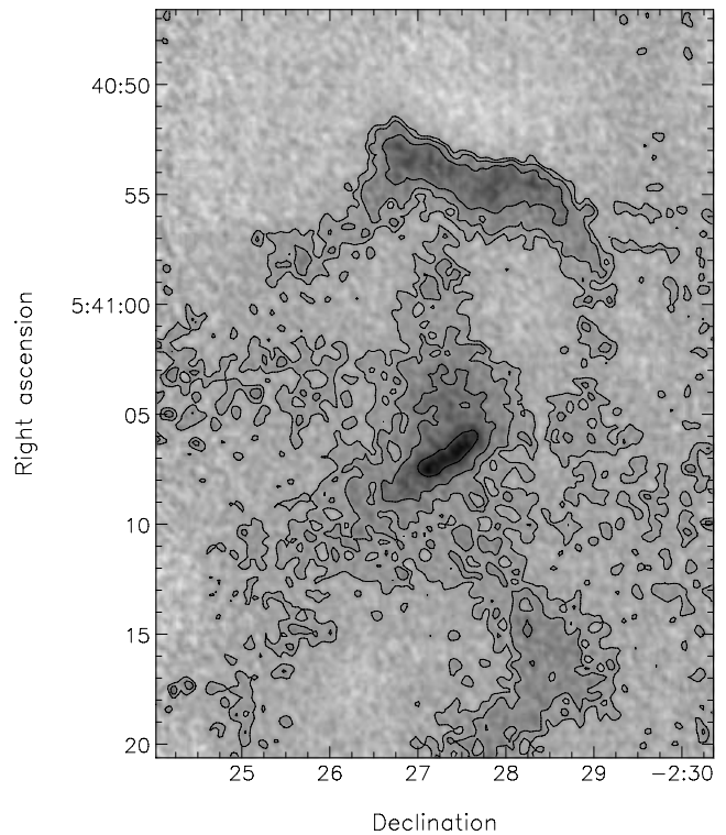
Figure 3. SCUBA 450- \mu\text{m} image of the Horsehead nebula. The same region is shown as in Fig. 2 and in the same orientation. Contour levels are again at 2, 3, 5 and 10\sigma , where 1\sigma is now 110 \text{ mJy beam}^{-1} . The FWHM beam size is 10 arcsec. The signal-to-noise ratio is lower than in the 850- \mu\text{m} image, although the horse’s head shape can still be made out. Once again the source associated with the PDR, SMM1, and the source in the throat, SMM2, can be seen.
