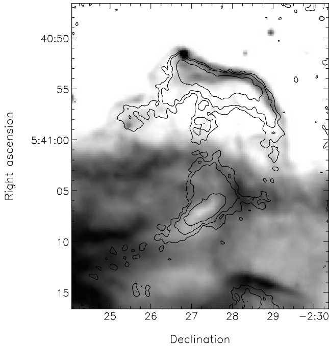
Figure 4. SCUBA 850- \mu\text{m} isophotal contour map of the Horsehead nebula overlaid on a grey-scale of the ISOCAM 6.75- \mu\text{m} image. The region shown is the same as that in Fig. 2. West is towards the top, north is to the left-hand side. Contour levels are as in Fig. 2. The submillimetre emission from the source SMM1 can now be seen to be offset from the infrared emission, with the latter lying closer to the H II region and appearing almost to wrap around the submillimetre source. The source SMM2 in the horse’s throat can be seen to be associated with a dip in the mid-infrared emission (cf. Abergel et al. 2003).
