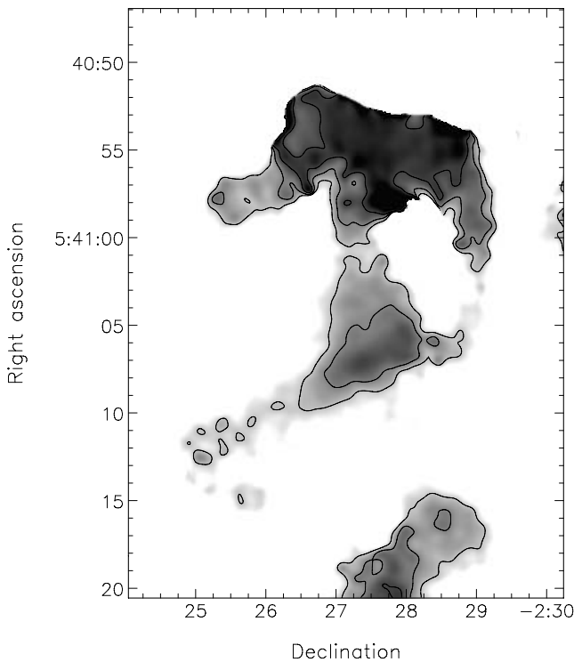
Figure 6. Image of the ratio of the 850- to 450- \mu\text{m} images shown in Figs 2 and 3 (after smoothing to a common resolution). Contour levels are 0.1, 0.2 and 0.3.
