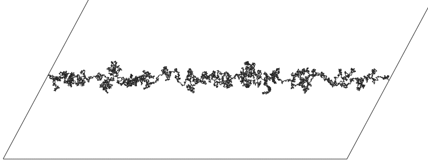
Figure 5: Localization of the front ( 2N = 500 , \ell_N = 1000 )
