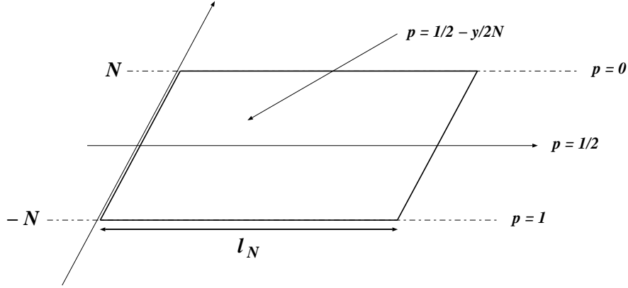
Figure 4: The strip where the percolation parameter p varies
