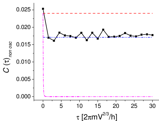
FIG. 6: (Color online) Correlation function \mathcal{C}_{\text{non osc}} of the quantity \varphi_{\text{non osc}} defined in Eq.(37) calculated from the simulation (square symbols; the solid line is a guide to the eye), or using the Gaussian theory (purple dashed-dotted line going to zero at long times). In dashed line (red) the Bogoliubov prediction. In dashed-dotted-dotted line (blue) the long time prediction (42) of the ergodic theory. The parameters T , N and \rho g have the same values as in Fig.1.
