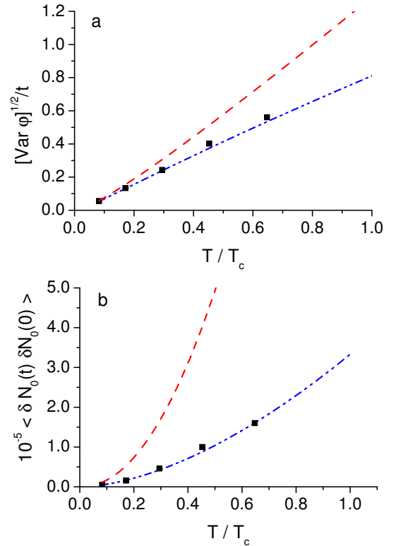
FIG. 5: (Color online) (a) Long time limit of (\text{Var } \varphi)^{1/2}/t , in units of \hbar/mV^{2/3} , as a function of the temperature over the ideal gas critical temperature. (b) Long time limit of the condensate atom number correlation function, as a function of T/T_c . In square symbols the numerical results of the classical field simulation (averaged over 500 realizations), in dashed line (red) the Bogoliubov prediction and in dashed-dotted (blue) the ergodic prediction. The parameters N and \rho g have the same values as in Fig.1.
