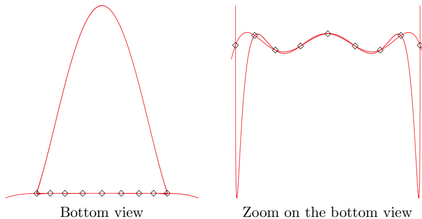
Figure 7: Knot K_9
