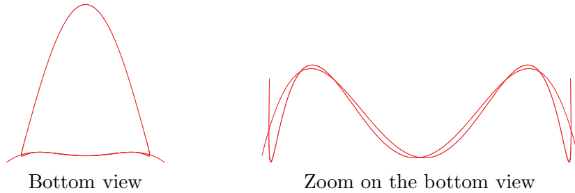
Figure 5: Knot K_7
