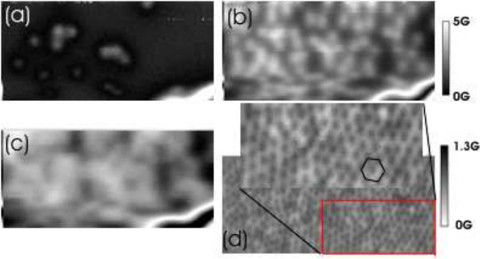
Fig. 2. Comparison between \text{NbSe}_2 and \text{Sr}_2\text{RuO}_4 for magnetic fields applied perpendicular to the ab plane. (a) A \mu\text{SFM} image after field cooling \text{Sr}_2\text{RuO}_4 in a field of 2 gauss, (b) in 6 gauss and (c) in 7 gauss. The imaging temperature is 0.35K for all images. Coalescence of vortices is observed. (d) A \mu\text{SFM} image of a vortex lattice in \text{NbSe}_2 . The data is acquired after field cooling the \text{NbSe}_2 crystal in 5 gauss at a temperature of 1.1K. The inset shows the hexagonal order of the lattice. For all images the imaging area is 62\mu\text{m} \times 30\mu\text{m} .
