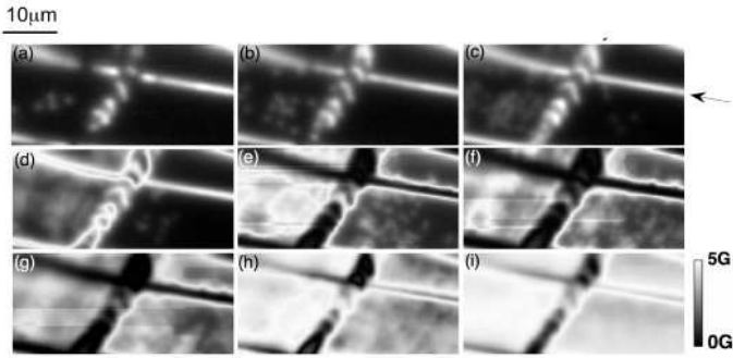
Fig. 2. Comparison between \text{NbSe}_2 and \text{Sr}_2\text{RuO}_4 for magnetic fields applied perpendicular to the ab plane. (a) A \mu\text{SFM} image after field cooling \text{Sr}_2\text{RuO}_4 in a field of 2 gauss, (b) in 6 gauss and (c) in 7 gauss. The imaging temperature is 0.35K for all images. Coalescence of vortices is observed. (d) A \mu\text{SFM} image of a vortex lattice in \text{NbSe}_2 . The data is acquired after field cooling the \text{NbSe}_2 crystal in 5 gauss at a temperature of 1.1K. The inset shows the hexagonal order of the lattice. For all images the imaging area is 62\mu\text{m} \times 30\mu\text{m} .
