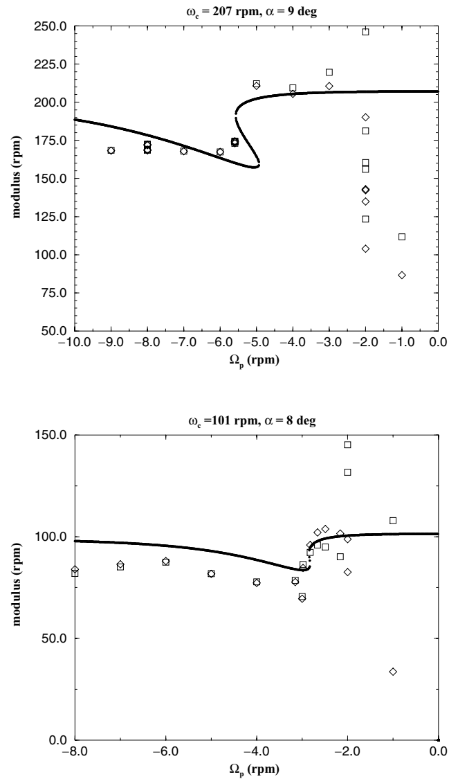
Figure 10. Rotation rate \omega_f of the fluid as a solid body. top: \omega_c = 207 rpm, \alpha = 9^\circ bottom: \omega_c = 101 rpm \alpha = 8^\circ .
