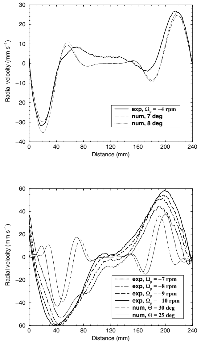
Figure 8. Comparison between measured and synthetic profiles of radial velocity using ultrasonic Doppler anemometry. \omega_c = 207 rpm, \alpha = 9^\circ top: \Omega = -4 rpm, bottom: \Omega \leq -7 rpm.
