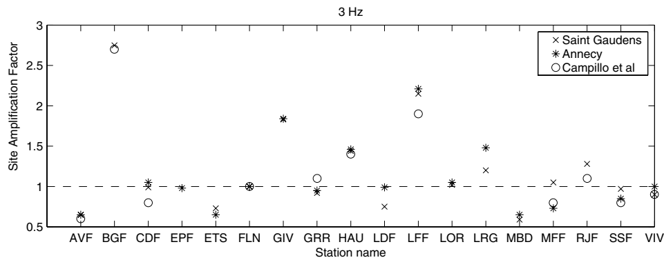
Figure 4. Comparison between the site amplification factors measured by Campillo et al. (1985) (O) and those obtained with the Saint-Gaudens (x) and Ancecy events (*).
