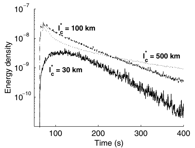
Figure 6. Synthetic coda envelope curves obtained with Monte Carlo simulations for different values of mean free path contrast between crust and mantle. The station is located 220 km away from the source. The mantle transport mean free path is 100 000 km and the crustal transport mean free path is 30 km (solid line), 100 km (dashed line) or 500 km (dotted line).
