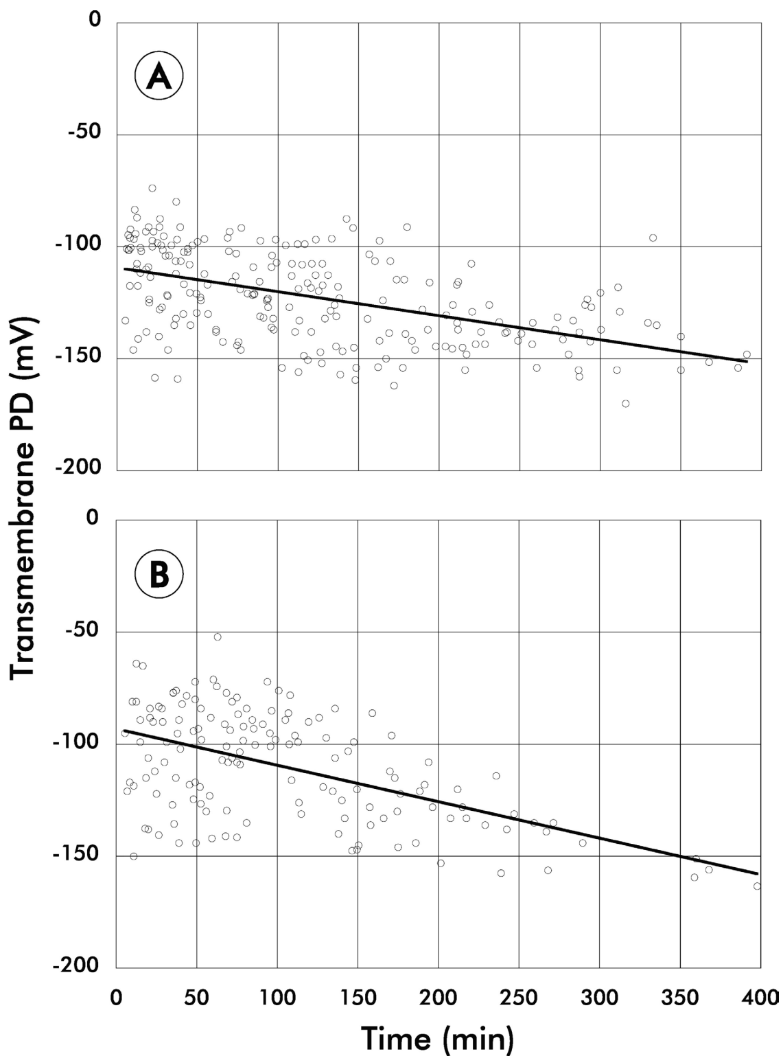
Figure 6. Effect of compound 9 on the transmembrane PD of subepidermal cells of Ricinus hook. A : control, the tissues were incubated in the standard medium (pH 5.0); B : treated set, the tissues were incubated in the same solution with compound 9 at 250 \mu M concentration. Linear regression was calculated with Kaleidagraph v. 3.5 software.
