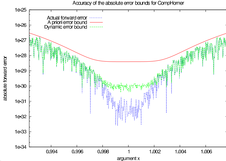
Figure 3: The dynamic error bound (20) compared to the a priori bound (13) and to the actual forward error ( p(x) = (1 - x)^5 for 400 entries on the x axis).
