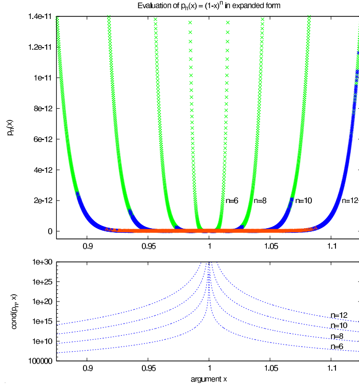
Figure 1: We report the evaluation of polynomials p_n near the multiple root x = 1 with the compensated Horner algorithm ( CompHornerIsFaithful ) and for multiplicity n = 6, 8, 10, 12 . Each evaluation proved to be faithfully rounded thanks to the dynamic test is reported with a green cross. The faithful evaluations that are not detected to be so with the dynamic test are represented in blue. Finally, the evaluations that are not faithfully rounded are reported in red. The lower frame represents the condition number with respect to the argument x .
