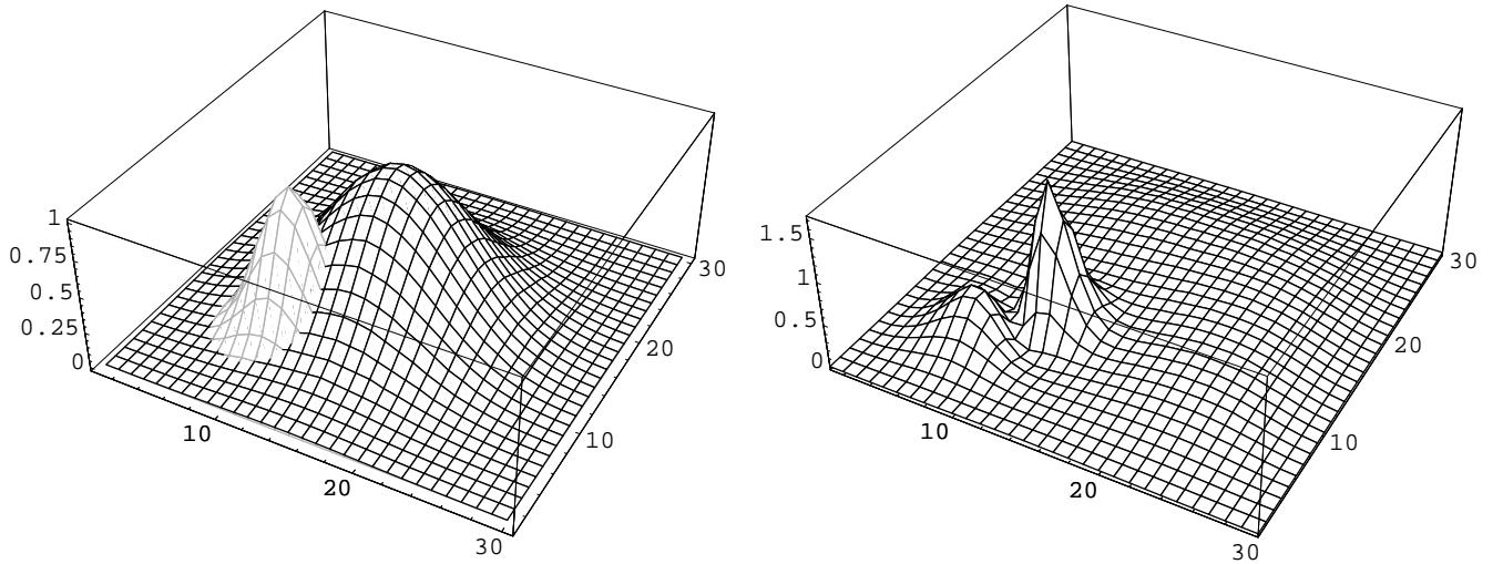
FIG. 1: Left : laser beam Gaussian profile to be coupled in the waveguide (black) and waveguide (gray) (A.U.). Right : beam profile after a 3mm propagation. The window size is 30\mu\text{m} and the beam wavelength is 250\mu\text{m} . The highest peak on the right evidences the light which is coupled into the waveguide.
