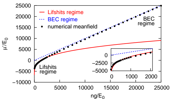
Figure 3: (color online) Chemical potential of a Bose gas in a speckle random potential with the same parameters as in Fig. 2 in the case of a tight radial confinement ( \mu' - \epsilon_\nu \ll \hbar\omega_\perp ). The points correspond to numerical calculations and the lines to the analytic formulae in both Lifshits [Eq. (16)] and BEC regimes [Eq. (13)].
