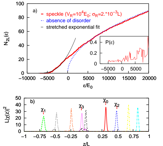
Figure 2: (color online) a) Cumulative density of states of single-particles in a speckle random potential. Inset: Participation ratio. b) Low-energy Lifshits eigenstates. Here E_0 = \hbar^2/2mL^2 .
