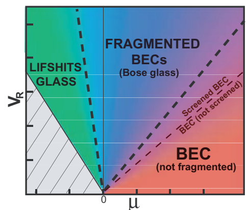
Figure 1: (color online) Schematic phase diagram of an ultracold Bose gas in a 1D random potential. The dashed lines represent the boundaries (corresponding to crossovers ) identified in this work and are controlled by the parameter \alpha_R = \hbar^2/2m\sigma_R^2V_R (see text). The hatched part corresponds to a forbidden zone ( \mu < V_{\min} ).
